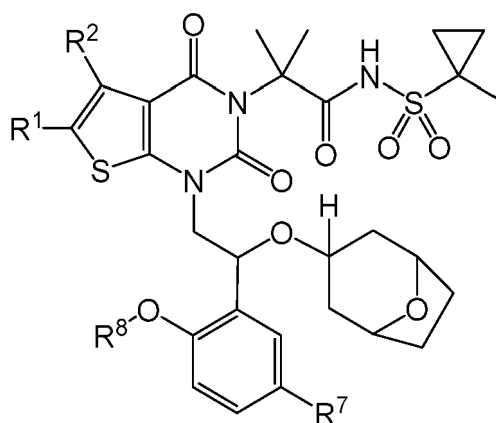
Formula (IV)
