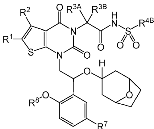
Formula (III)
