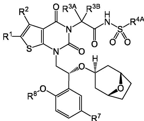
Formula (IIIa).
