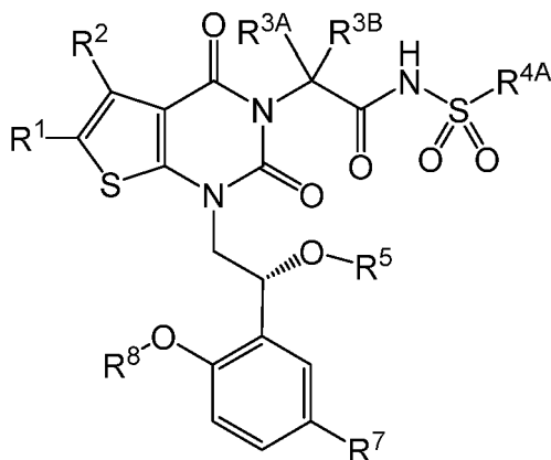
Formula (IIa)
