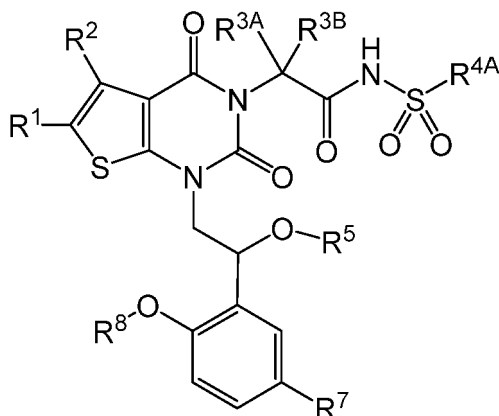
Formula (II)
