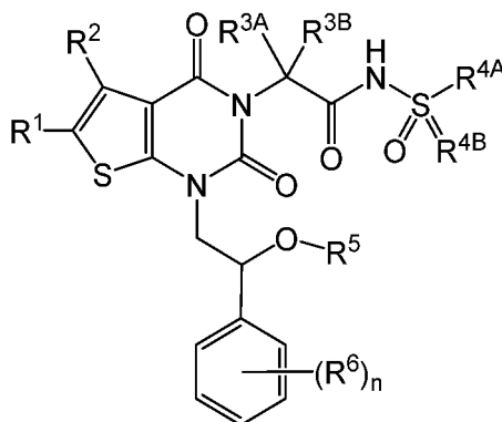
Formula I
