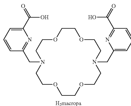
Scheme 1. Structures of \text{H}_2\text{macropa} , \text{H}_2\text{macropa-NCS} ("macropa-ncs"), and \text{macropa}-(\text{OCH}_2\text{CH}_2)-\text{Ph}-\text{NCS} .
