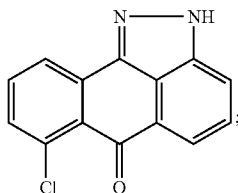
7-Chloro-2H-dibenzo[cd,g] indazol-6-one
