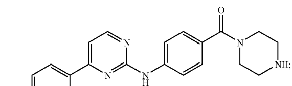
{4-[4-(4-Chloro-phenyl)-pyrimidin-2-ylamino]-phenyl}-piperazin-1-yl-methanone
