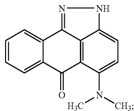
5-Dimethylamino-2H- dibenzo[cd,g]indazol-6-one
