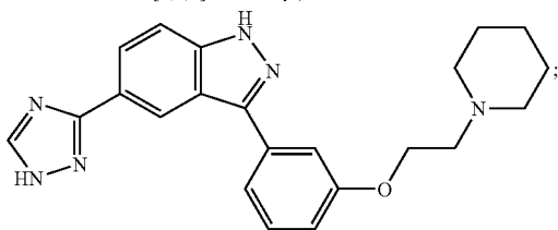
3-[3-(2-Piperidin-1-yl-ethoxy)-phenyl]-5-(1H-[1,2,4]triazol-3-yl)-1H-indazole
