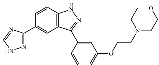
3-[3-(2-Morpholin-4-yl-ethoxy)-phenyl]-5-(1H-[1,2,4]triazol-3-yl)-1H-indazole
