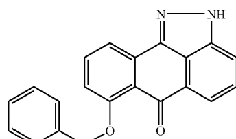
7-Benzyloxy-2H-dibenzo[cd,g]indazol- 6-one
