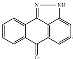
2H-Dibenzo[cd,g] indazol-6-one
