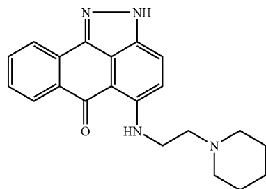
5-(2-Piperidin-1-yl-ethylamino)-2H- dibenzo[cd,g]indazole-6-one
