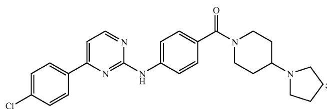
{4-[4-(4-Chloro-phenyl)-pyrimidin-2-ylamino]-phenyl}-(4-pyrrolidin-1-yl-piperidin-1-yl)-methanone
