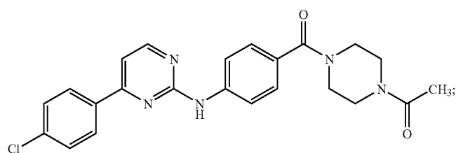
1-[4-{4-[4-(4-Chloro-phenyl)-pyrimidin-2-ylamino]-benzoyl}-piperazin-1-yl]-ethanone
