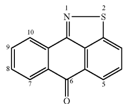
Anthra[9,1-cd]isothiazol-6-one
