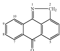
2H-Dibenzo[cd,g]indol-6-one
