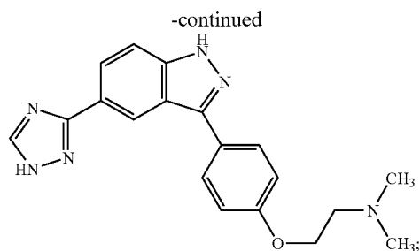
Dimethyl-(2-{4-[5-(1H-[1,2,4]triazol-3-yl)-1H-indazol-3-yl]-phenoxy}-ethyl)-amine
