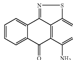
5-Amino-anthra[9,1- cd]isothiazol-6-one
