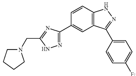
3-(4-Fluoro-phenyl)-5-(5-pyrrolidin-1-ylmethyl-1H-[1,2,4]triazol-3-yl)-1H-indazole
