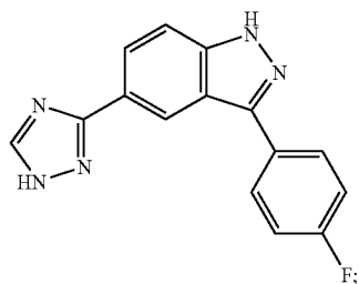
3-(4-Fluoro-phenyl)-5-(1H-[1,2,4]triazol-3-yl)-1H-indazole
