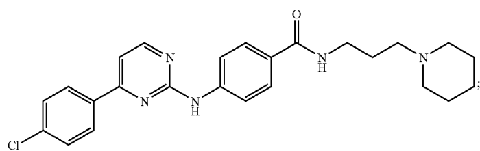
4-[4-(4-Chloro-phenyl)-pyrimidin-2-ylamino]-N-(3-piperidin-1-yl-propyl)-benzamide
