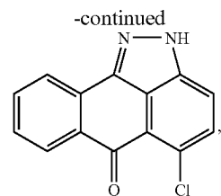
5-Chloroanthra[1,9-cd]pyrazol-6(2H)-one
