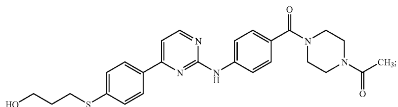
1-[4-{4-[4-(3-Hydroxy-propylsulfanyl)-phenyl]-pyrimidin-2-ylamino]-benzoyl}-piperazin-1-yl]-ethanone
