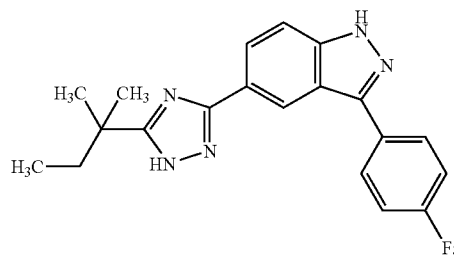
5-[5-(1,1-Dimethyl-propyl)-1H-[1,2,4]triazol-3-yl]-3-(4-fluoro-phenyl)-1H-indazole
