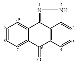
2H-Dibenzo[cd,g]indazol-6-one
