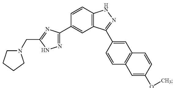
3-(6-Methoxy-naphthalen-2-yl)-5-(5-pyrrolidin-1-ylmethyl-1H-[1,2,4]triazol-3-yl)-1H-indazole
