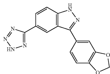
3-Benzo[1,3]dioxol-5-yl-5-(2H-tetrazol-5-yl)-1H-indazole
