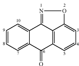
2-Oxa-1-aza-acanthrylen-6-one
