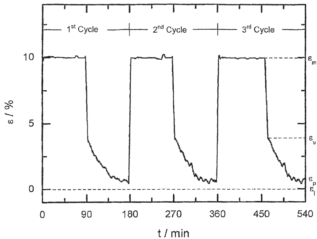
Elongation \varepsilon of a photosensitive network (Sample 7A) during 3 repetitions of a photomechanical cycle (stress regulated)
