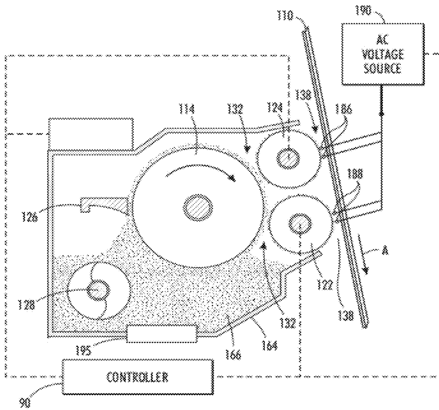
FIG. 1 PRIOR ART
