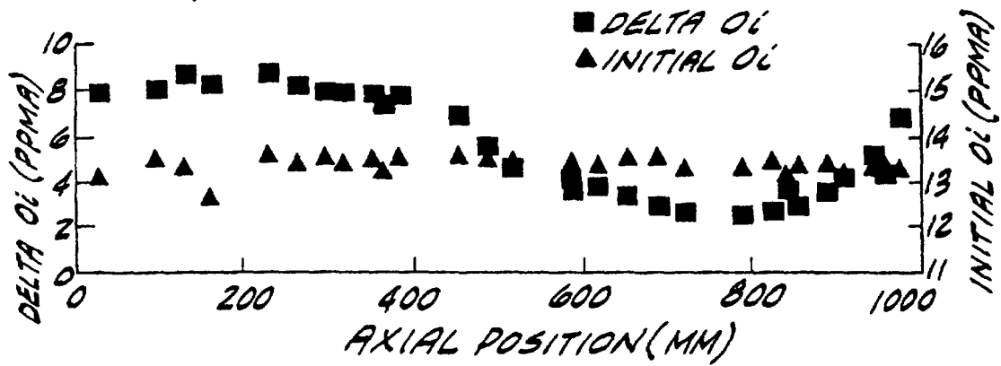
FIG. 9a OXYGEN PRECIPITATION (CONVENTIONAL PROCESS)
