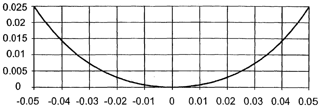
COSH Dimple Profile a=40, r=0.05, d=0.025, vr=0.55
