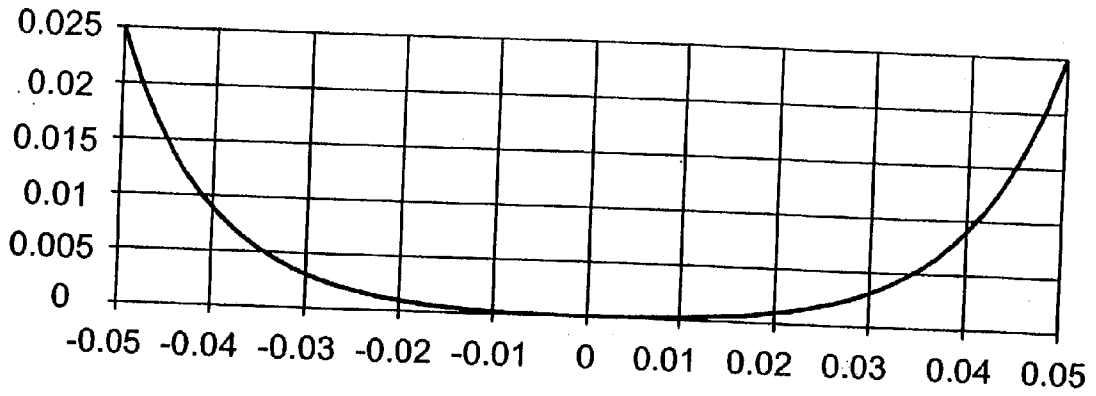
COSH Dimple Profile a=100, r=0.05, d=0.025, \nu r=0.69
