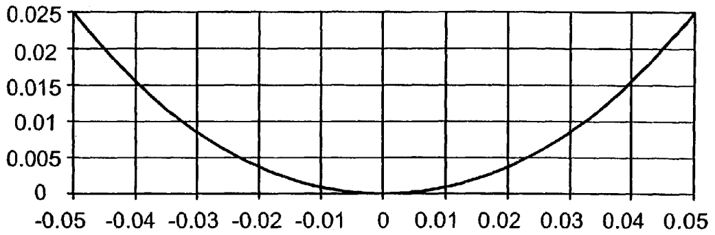
COSH Dimple Profile a=20, r=0.05, d=0.025, vr=0.51
