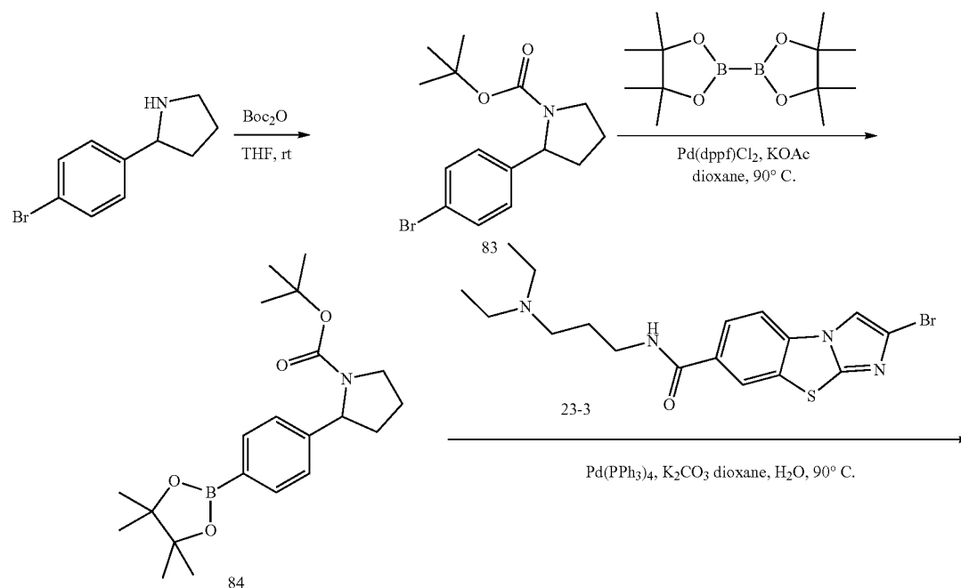
Scheme 55
