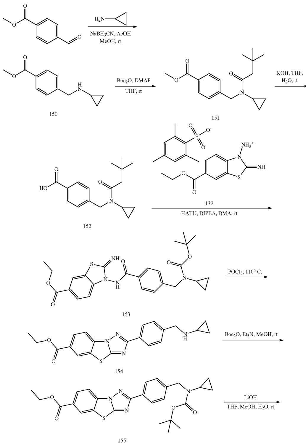
Scheme 71
