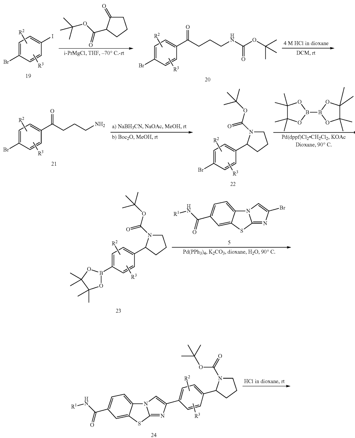
Scheme 15.
