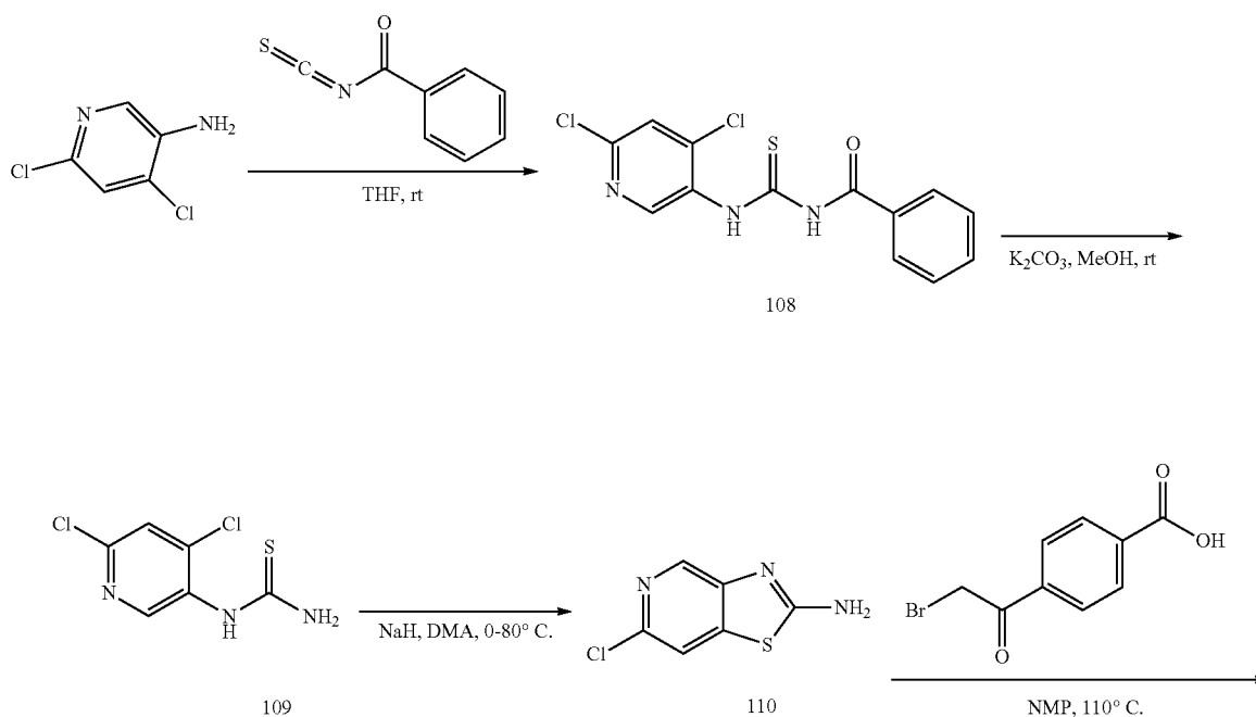
Scheme 61
