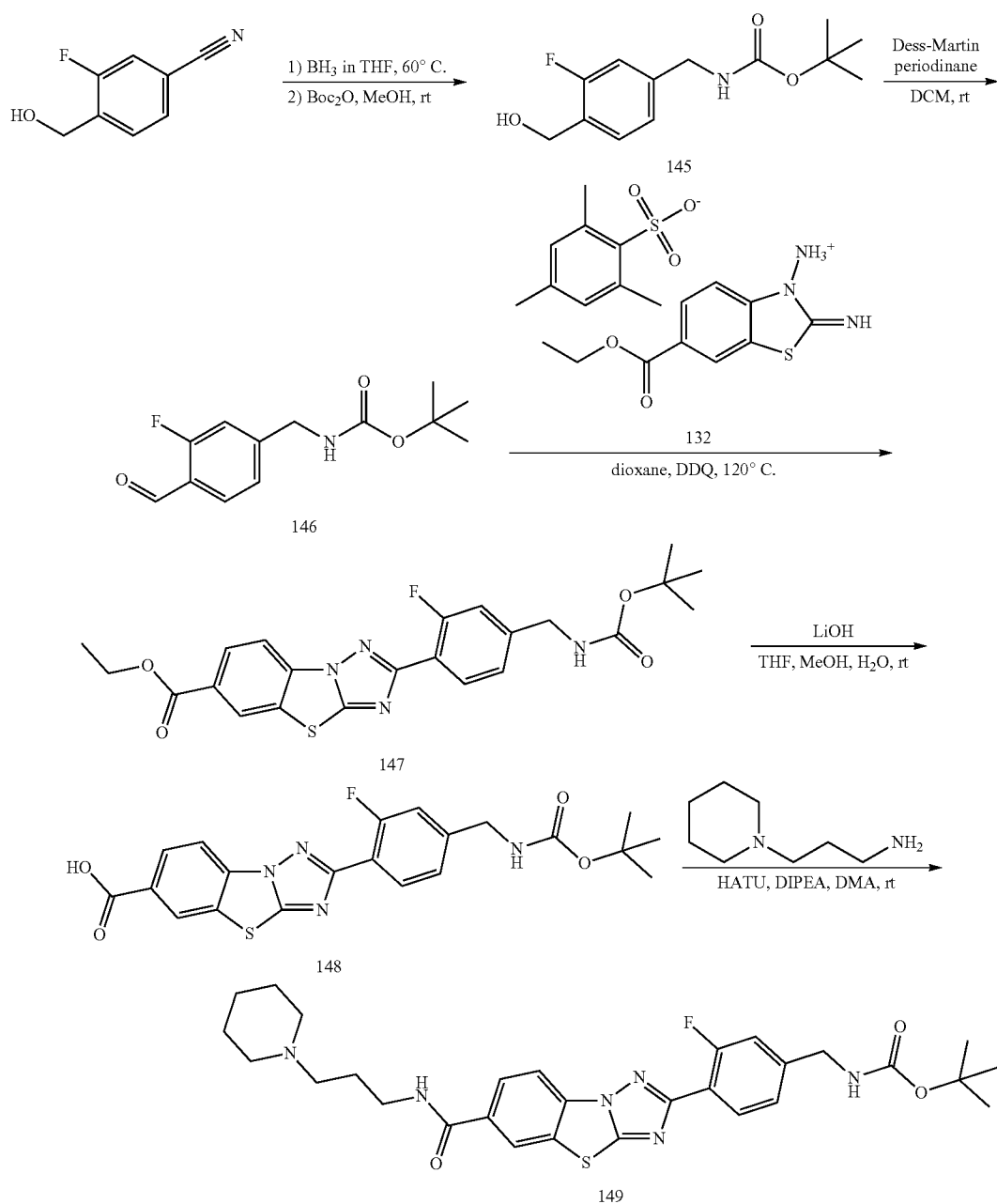
Scheme 70
