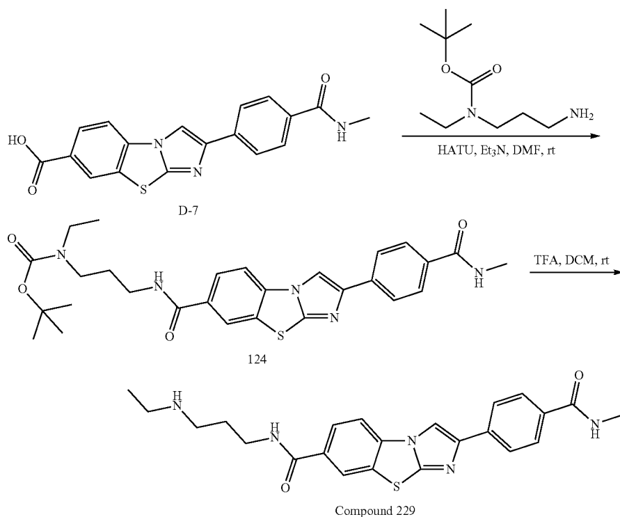
Scheme 65
