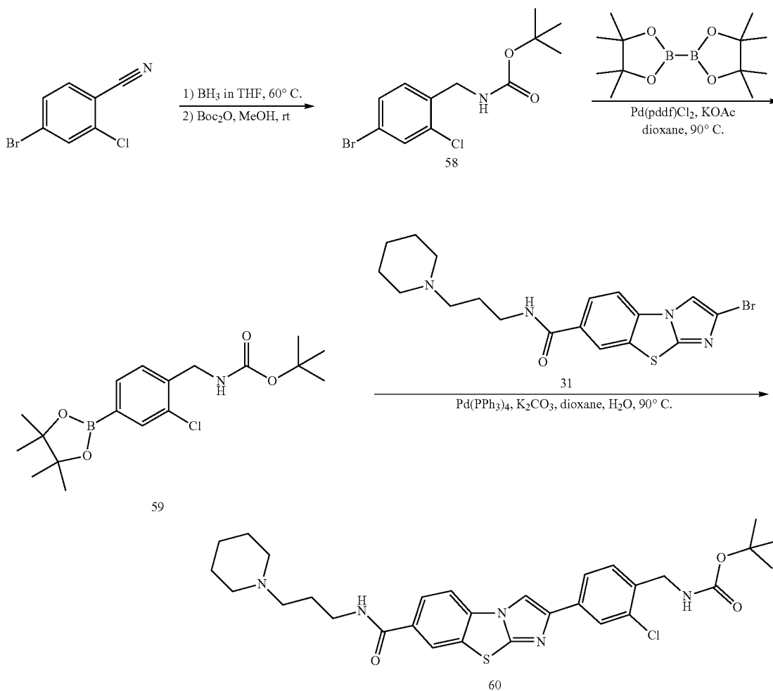
Scheme 49
