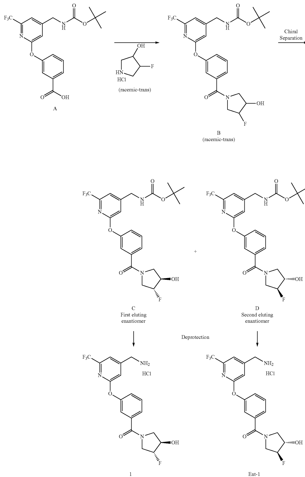
Scheme 1. Preparation via Chiral Separation
