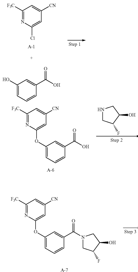
Scheme 3. Preparation of Compound 2.
