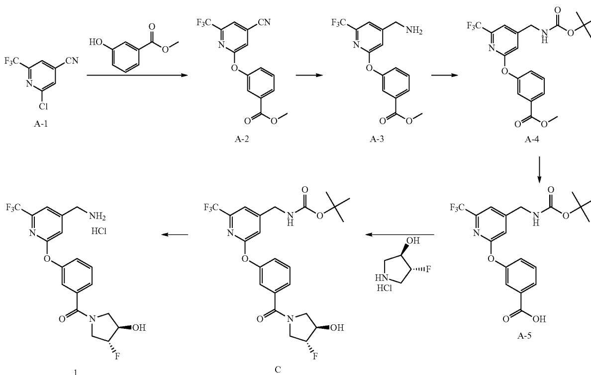
Scheme 2. Preparation of Compound 1 without Chiral Separation.
