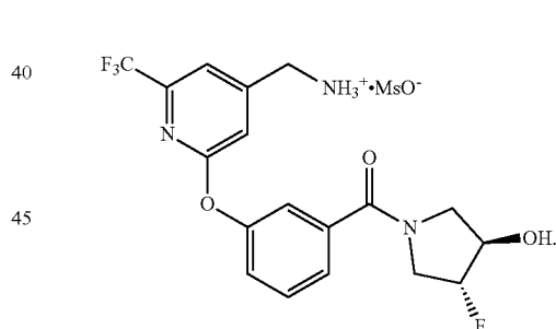
Compound 2
