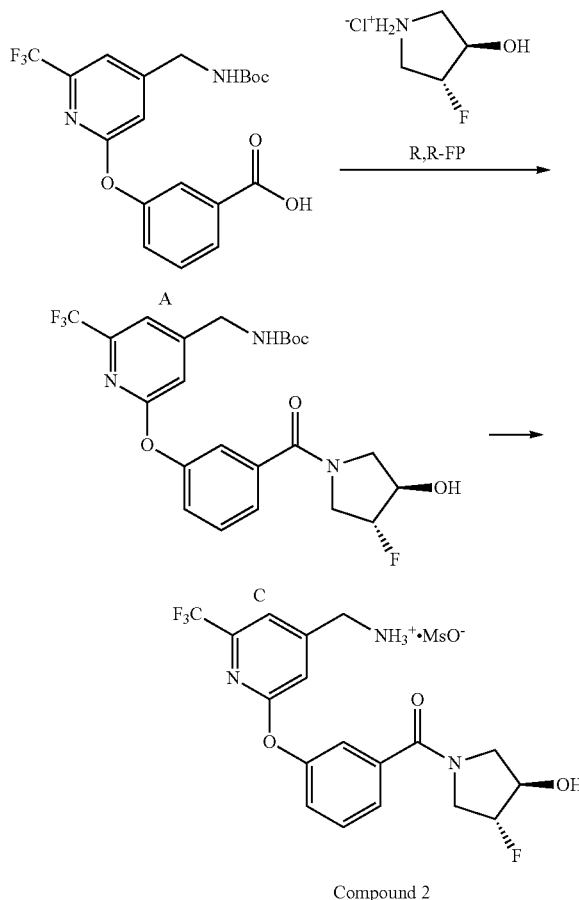
Scheme 4. Alternative Preparation of Compound 2.
