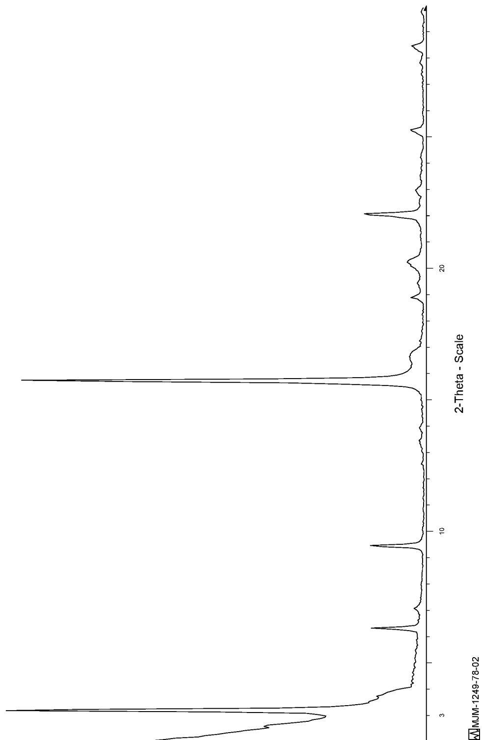
FIGURE 3 XRPD of Compound 2, Form 2
