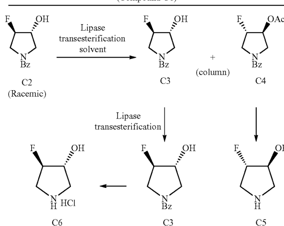
Scheme 5. Preparation of (3R,4R)-4-fluoropyrrolidin-3-ol, hydrochloride (Compound C6)
