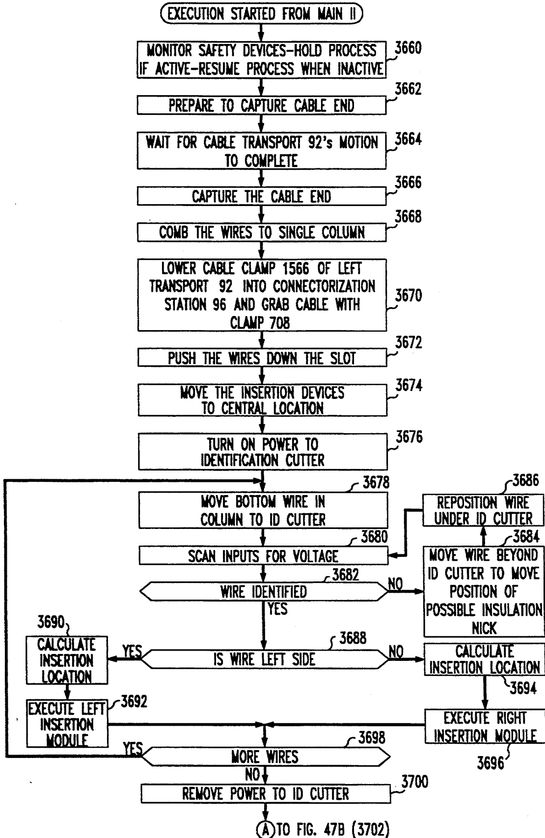
FIG. 47A IDENTIFY AND CONNECTORIZE II
