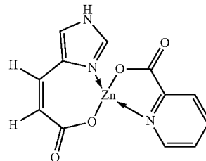
Zinc Urocanate Picolinate
