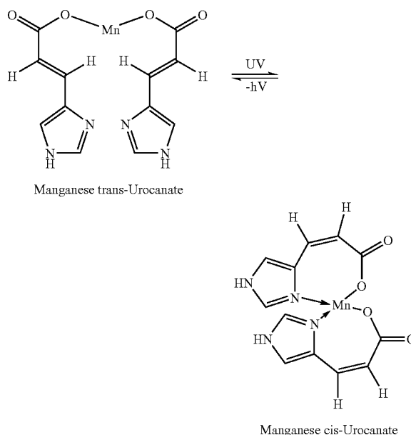
FIG. 4. Manganese Urocanate Photoisomerism
