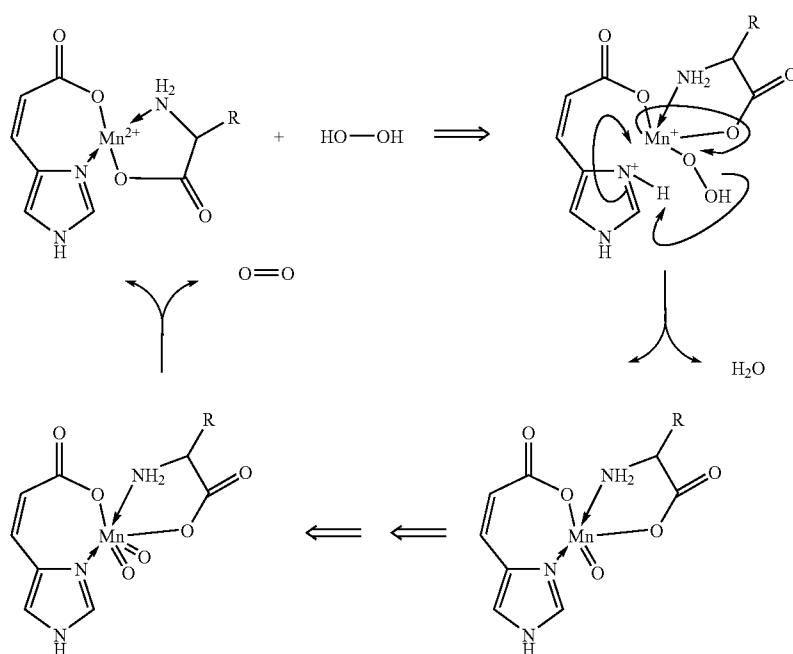
FIG. 6. Catalase Mimetic Decomposition of Peroxide by Manganese Complexes
