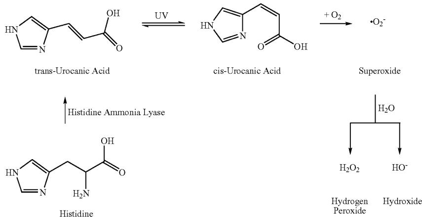
FIG. 2. Urocanate Pathway for Peroxide Formation
