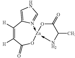
Zinc Urocanate Alaninate
