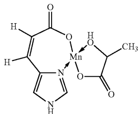
Manganese Urocanate Lactate
