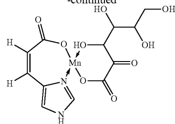
Manganese Urocanate Ascorbate (Alternate Structure)
