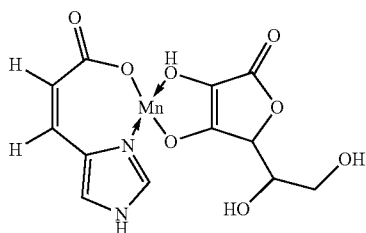
Manganese Urocanate Ascorbate
