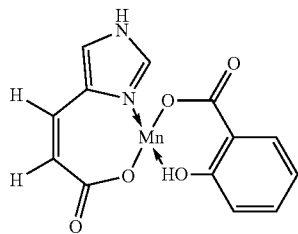
Manganese Urocanate Salicylate
