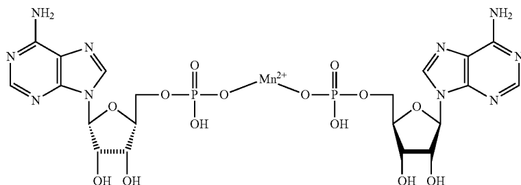
Manganese Adenosine Phosphate
