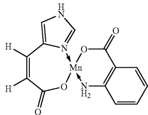
Manganese Urocanate Anthranilate
