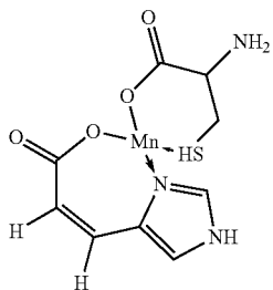
Manganese Urocanate Cysteinate
