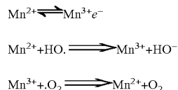
FIG. 3. Free Radical Scavenging by Manganese Ions
