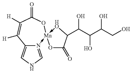
Manganese Urocanate Gluconate
