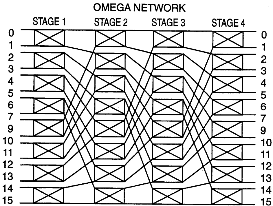
FIG. 1C PRIOR ART
