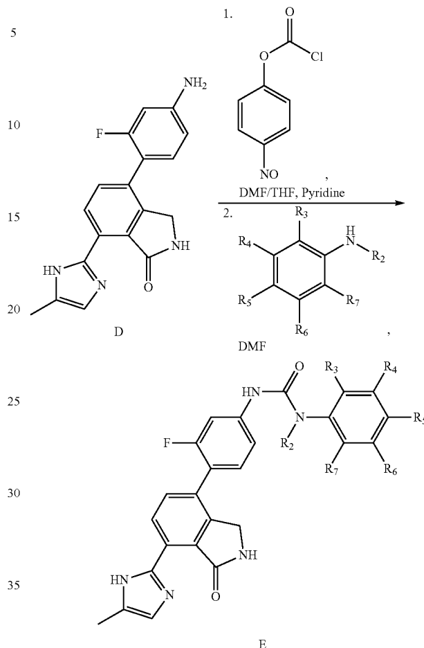
[Reaction Scheme 2]
