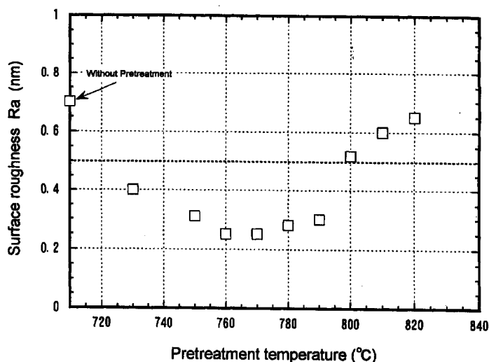
Dependency of Surface roughness of crystallized glass (Example 1) on Pretreatment temperature
