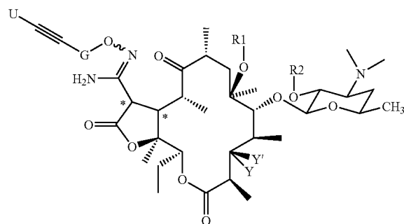
XXIIa, Y' is H, Y is Ocladinose, R2, R2' is TES
