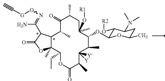
XXIIa, Y' is H, Y is Ocladinose, R2, R2' is TES
