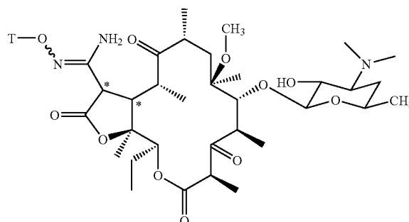
Formula I-f
