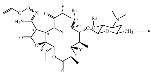
XVIIIa, Y' is H, Y is Ocladinose, R2, R2' is TES
