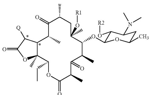
Formula I-d
