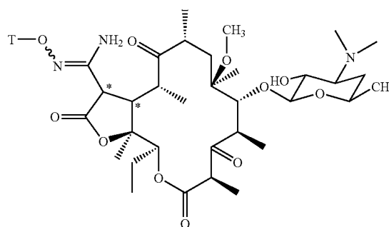
Formula I-f
