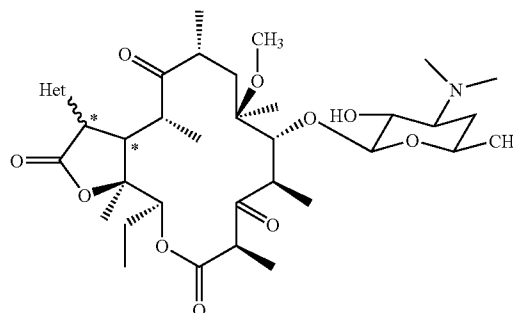
Formula I-e
