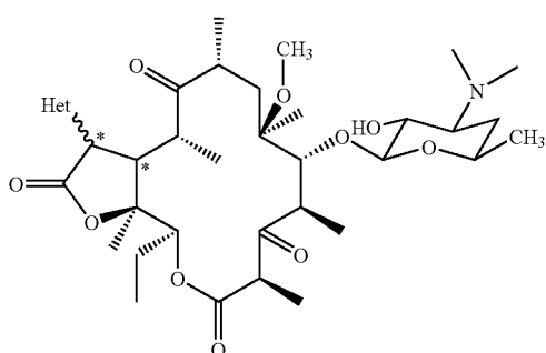
Formula I-e
