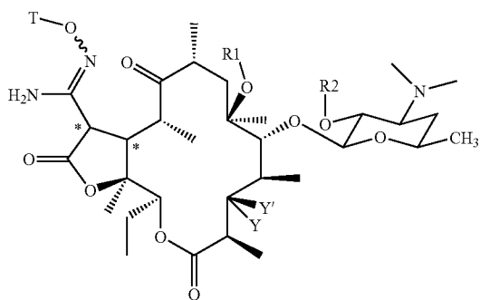
XXIVa, Y' is H, Y is Ocladinose, XXIVb, Y', Y together C = O
