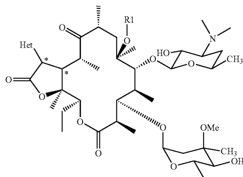
Formula I-b
