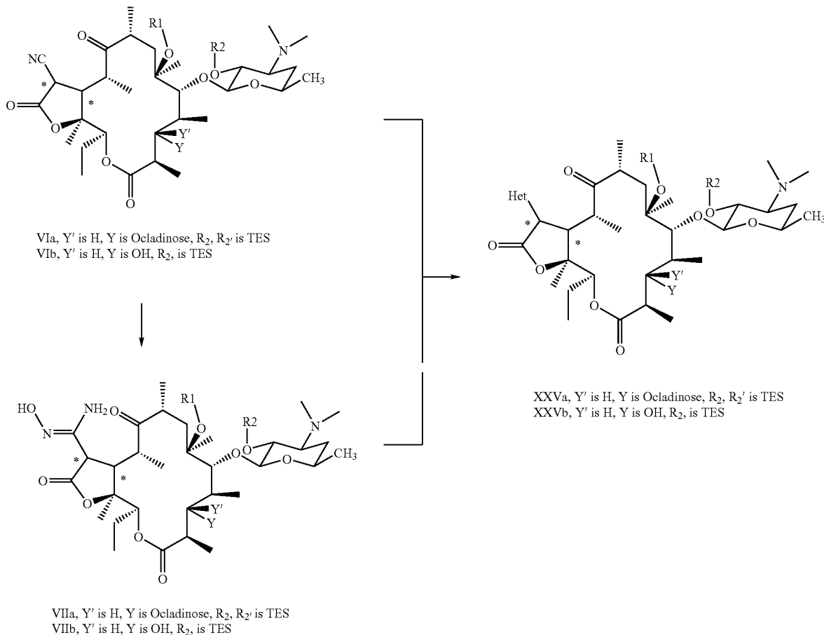
Scheme 9
