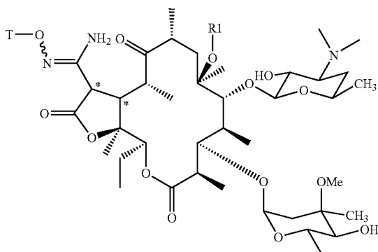
Formula I-c
