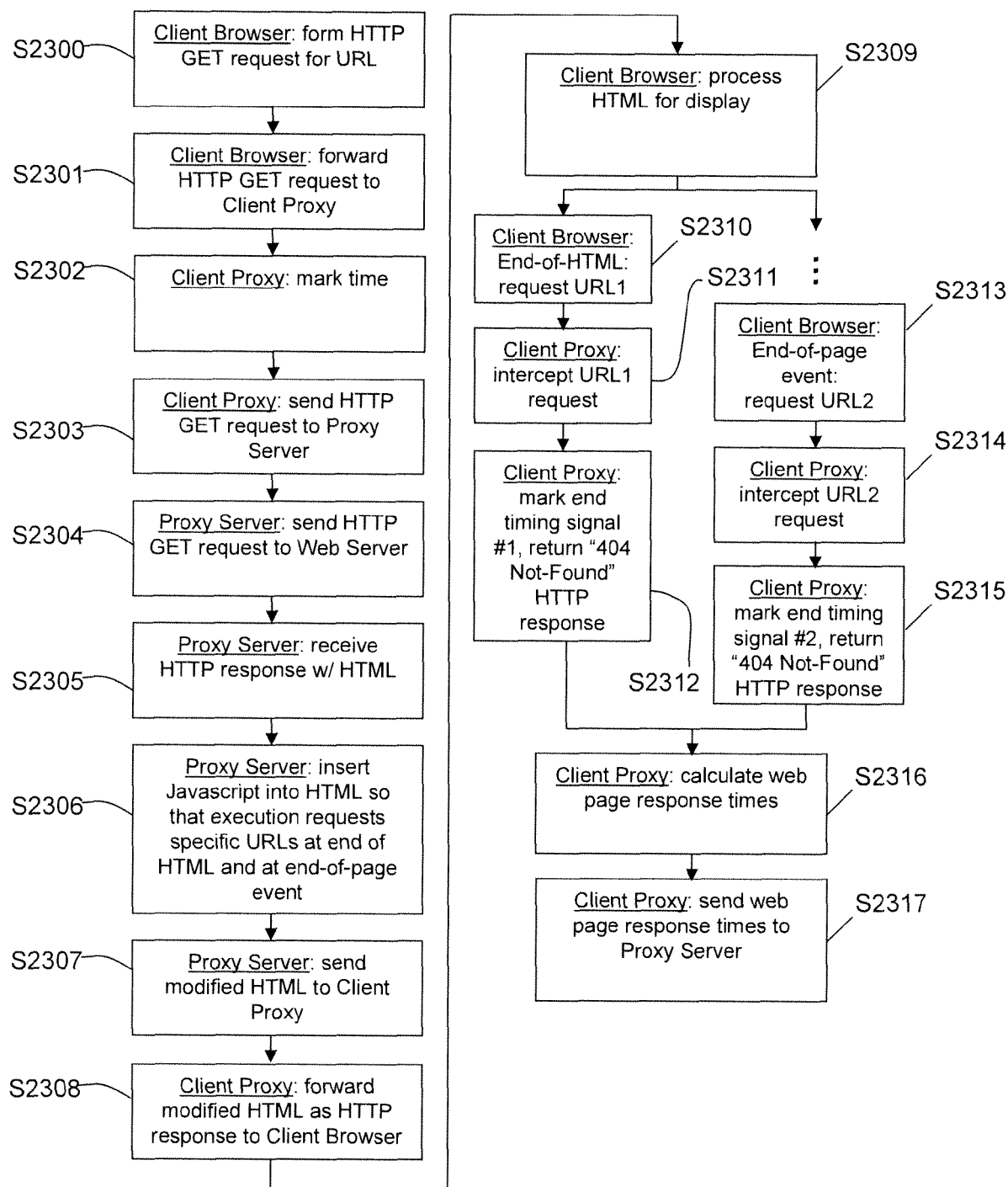
Fig. 23 Web Page Response Time
