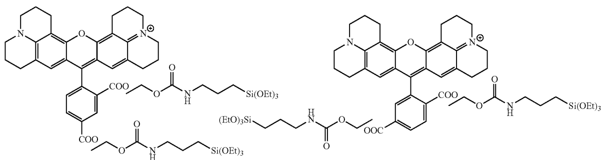
5- and 6-Carboxy X-rhodamine -Silylated
