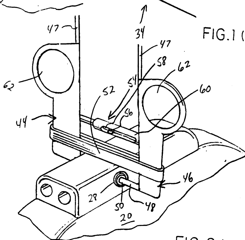
FIG. 2 (PRIOR ART)
