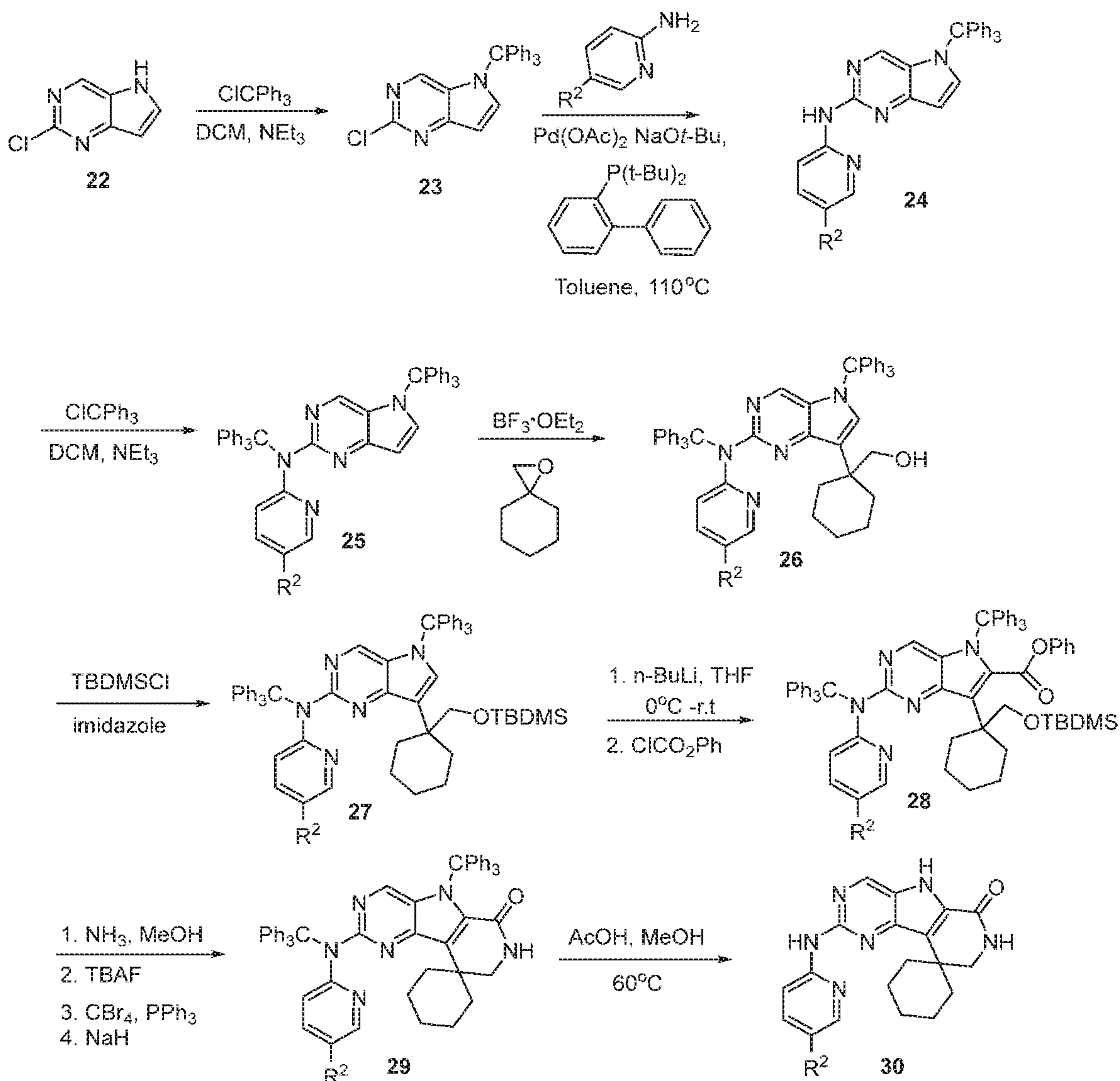
Scheme 4
