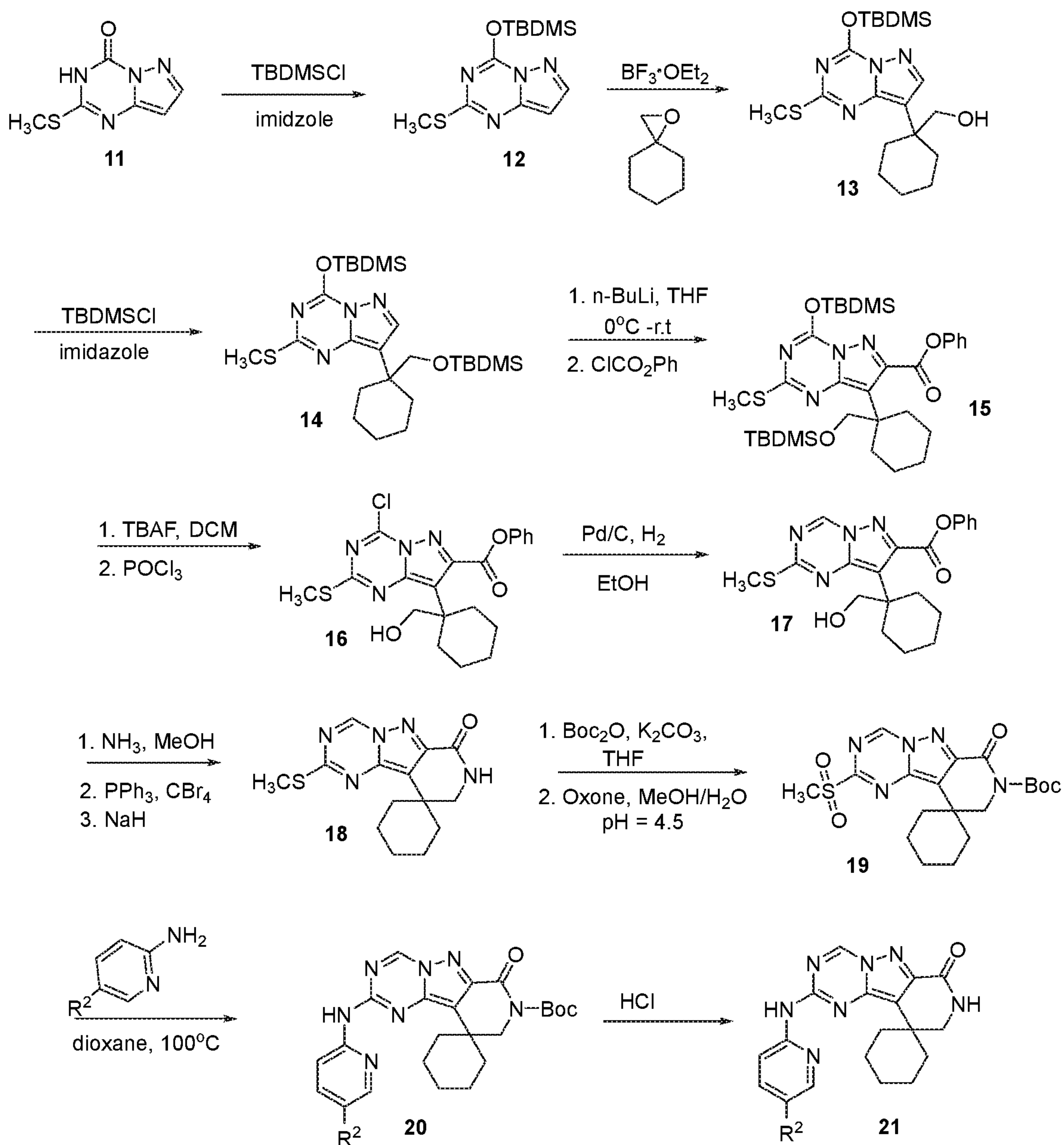
Scheme 3
