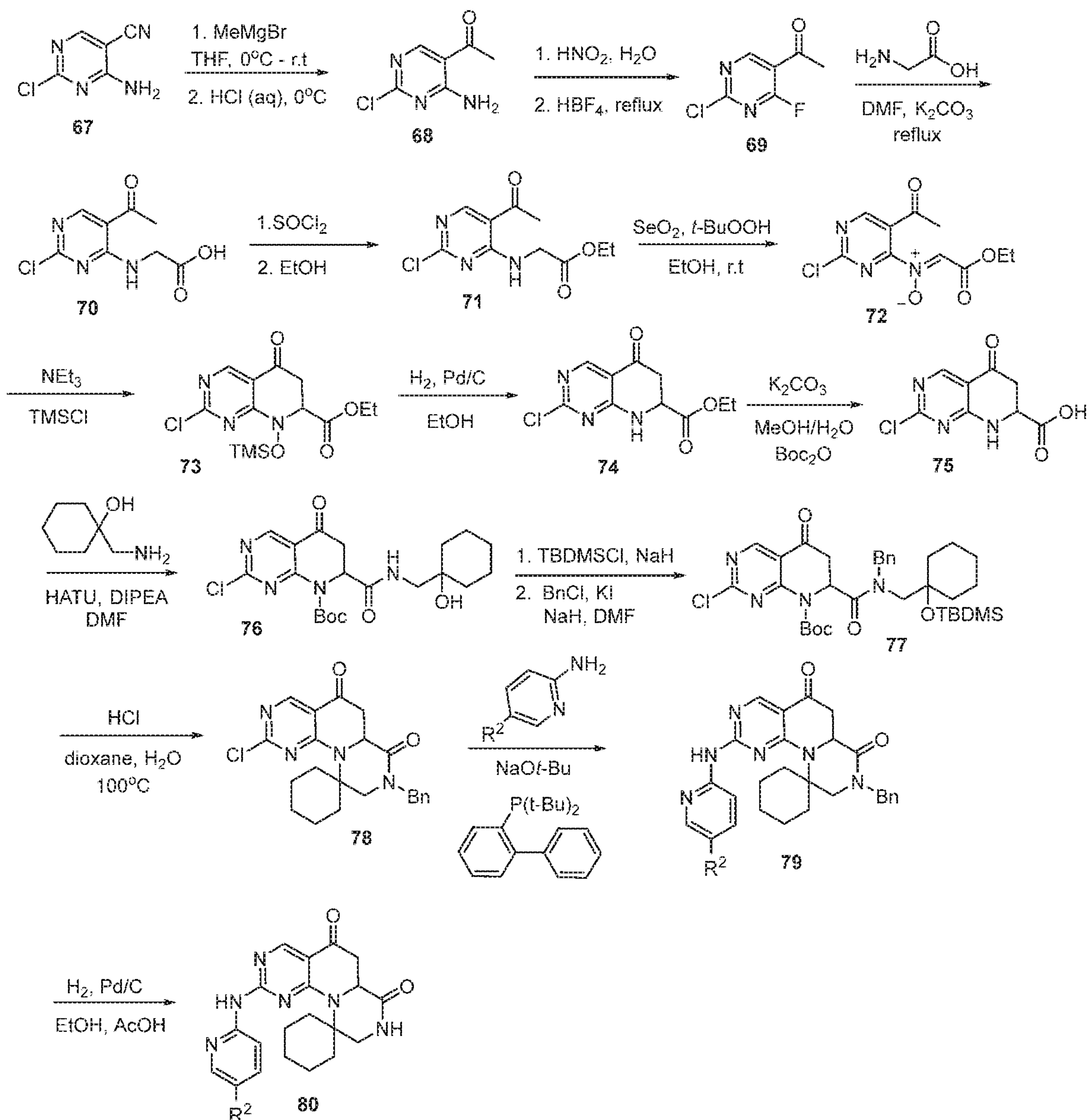
Scheme 9
