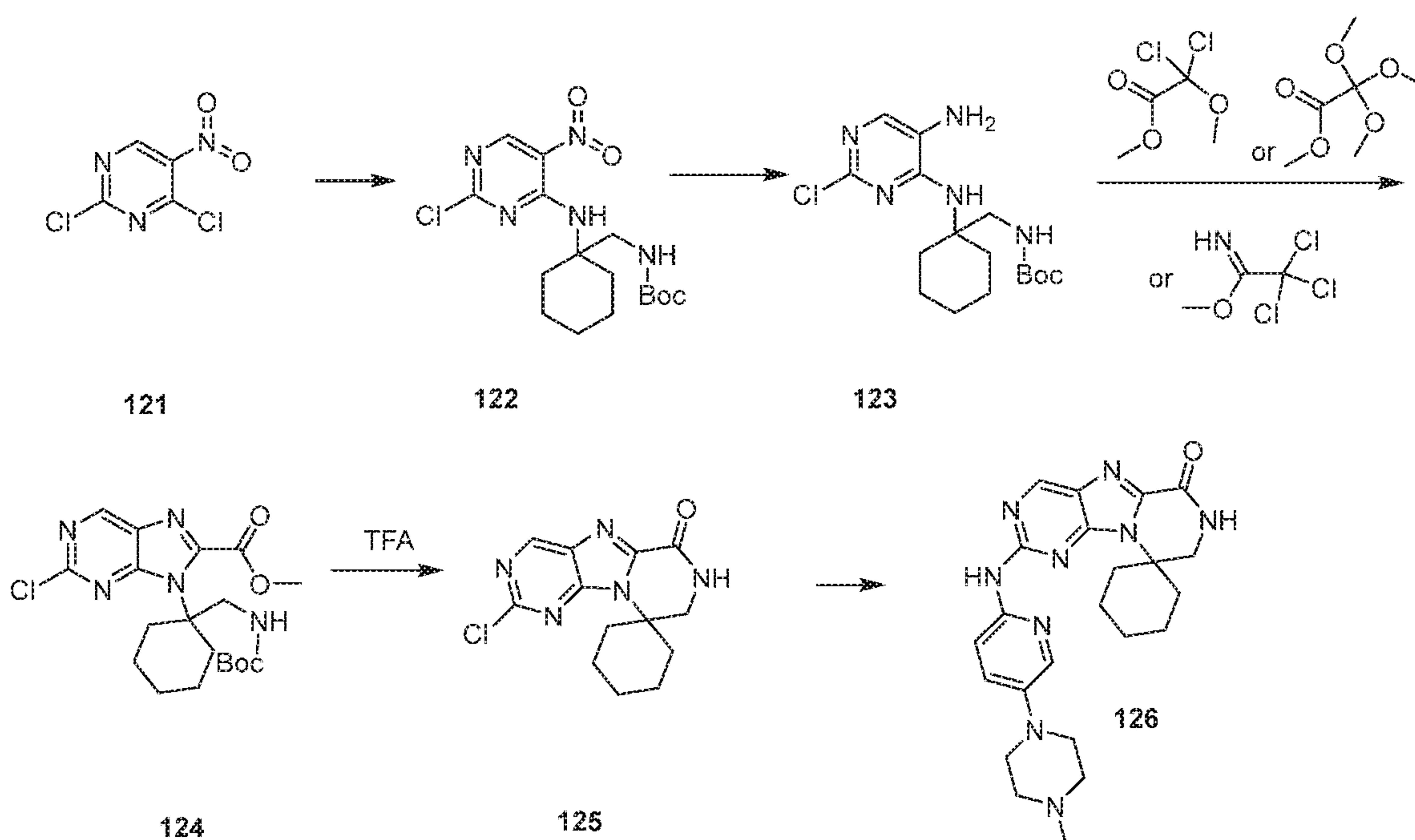
Scheme 18
