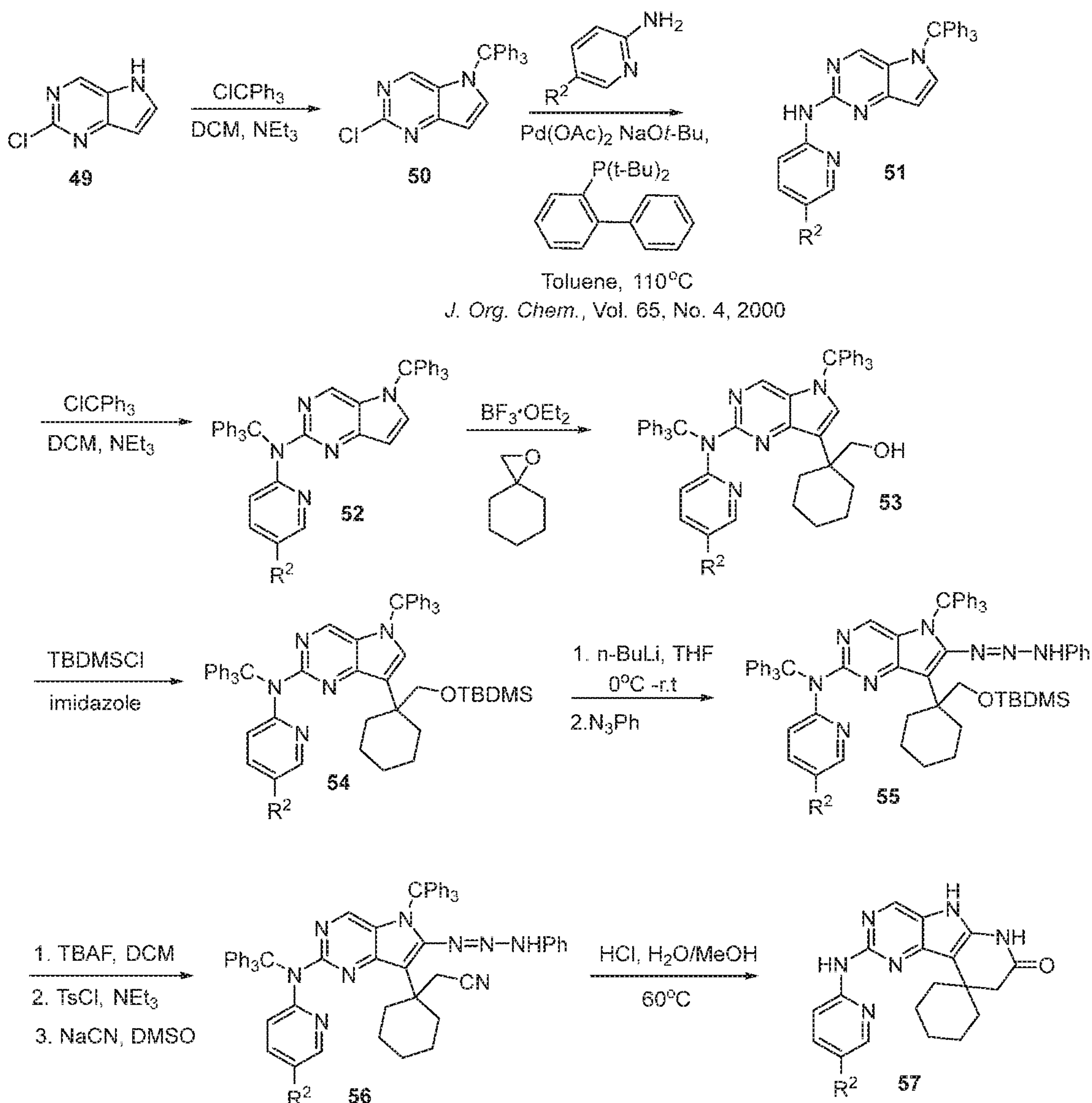
Scheme 7
