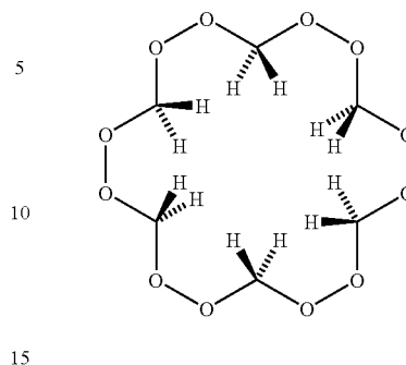
Scheme 8. An example of a cyclic tethered system
