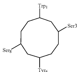
Scheme 10. Proposed cyclic decapeptides for proof of concept experiments.
