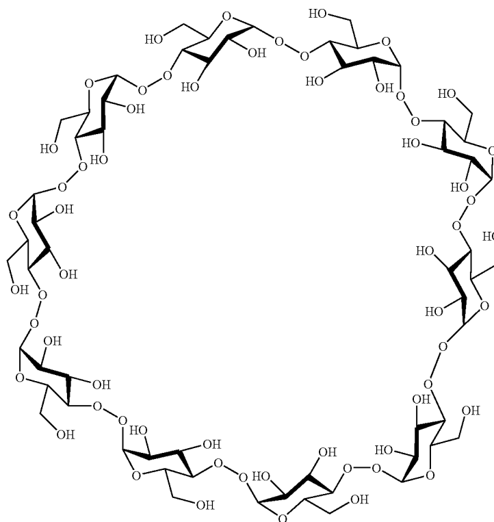
Scheme 9. A ten saccharide cyclodextrin
