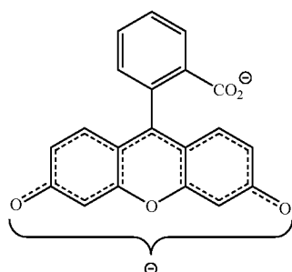
Scheme 13. Deprotonated and protonated forms of fluorescein shown delocalized
