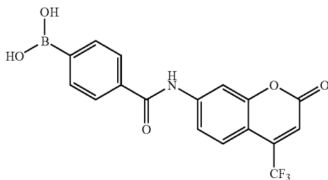
Argofluor-327d
