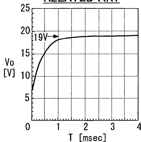
FIG. 7B RELATED ART
