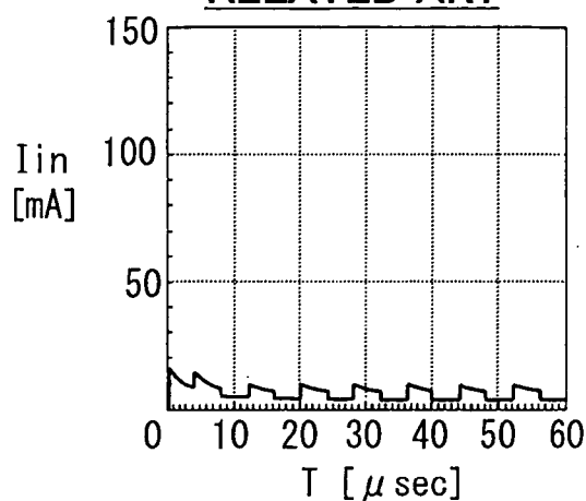
FIG. 10C RELATED ART
