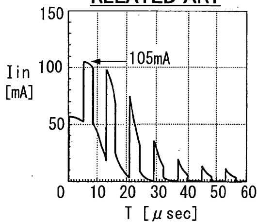
FIG. 7C RELATED ART
