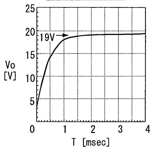
FIG. 10B RELATED ART
