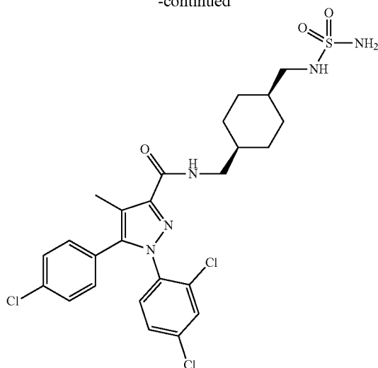
5-(4-chlorophenyl)-1-(2,4-dichlorophenyl)-4-methyl-N-(((1S,4S)-4-((sulfamoylamino)methyl)cyclohexyl)methyl)-1H-pyrazole-3-carboxamide
