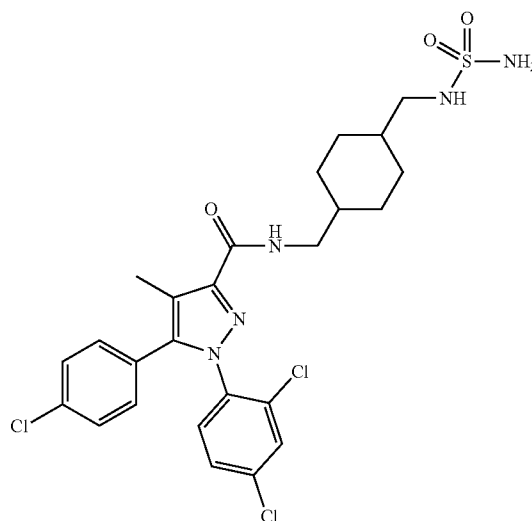
5-(4-chlorophenyl)-1-(2,4-dichlorophenyl)-4-methyl-N-((4-((sulfamoylamino)methyl)cyclohexyl)methyl)-1H-pyrazole-3-carboxamide
