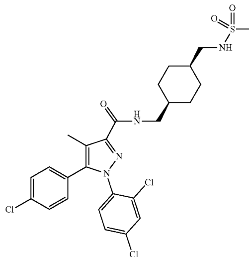
5-(4-chlorophenyl)-1-(2,4-dichlorophenyl)-4-methyl-N-(((1s,4s)-4-(methylsulfonamidomethyl)cyclohexyl)methyl)-1H-pyrazole-3-carboxamide
