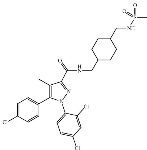
5-(4-chlorophenyl)-1-(2,4-dichlorophenyl)-4-methyl-N-((4-(methylsulfonamidomethyl)cyclohexyl)methyl)-1H-pyrazole-3-carboxamide
