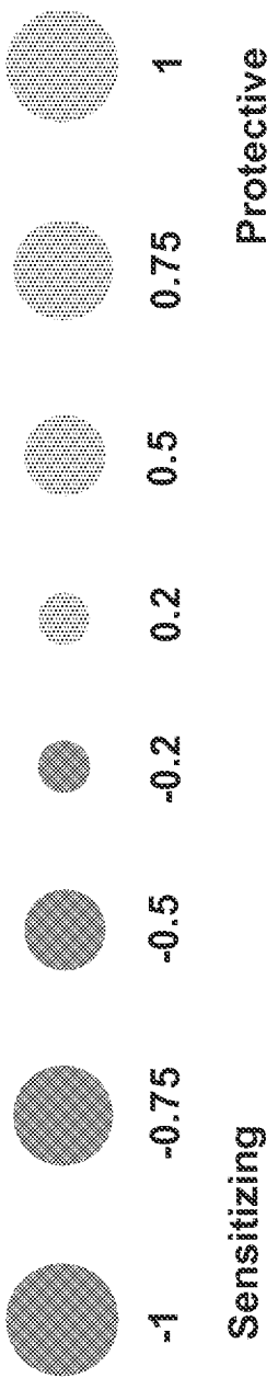
FIG. 13B-1 Gene phenotype (average of 3 most active sgRNAs)
