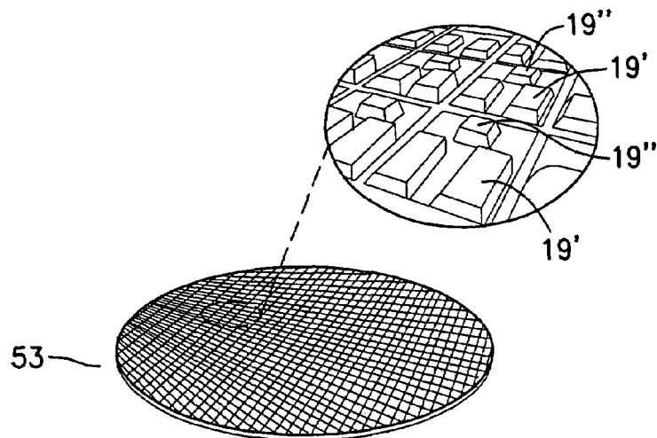
Fig. 17 Prior Art
