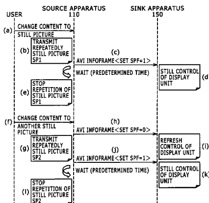
CONTROL SEQUENCE CHART
