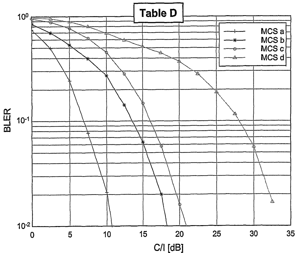
FIG.14 BLER versus C/I for a selection of MCS (high diversity, with IR)
