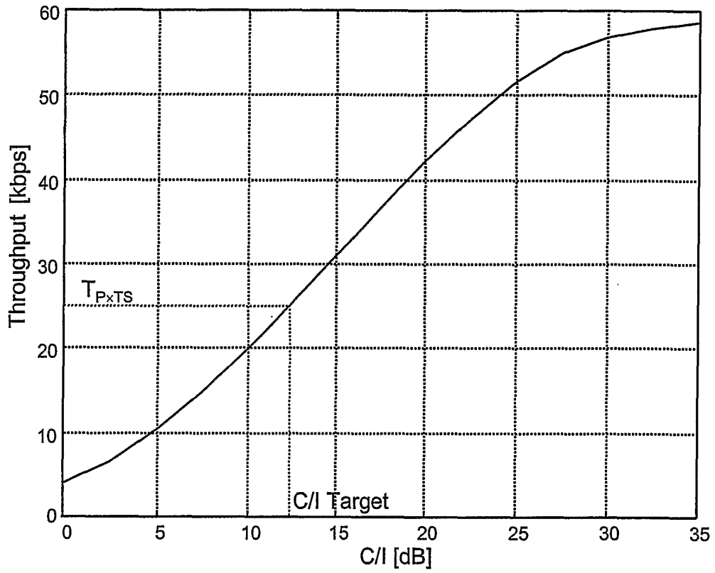
Maximum achievable throughput (with IR)
