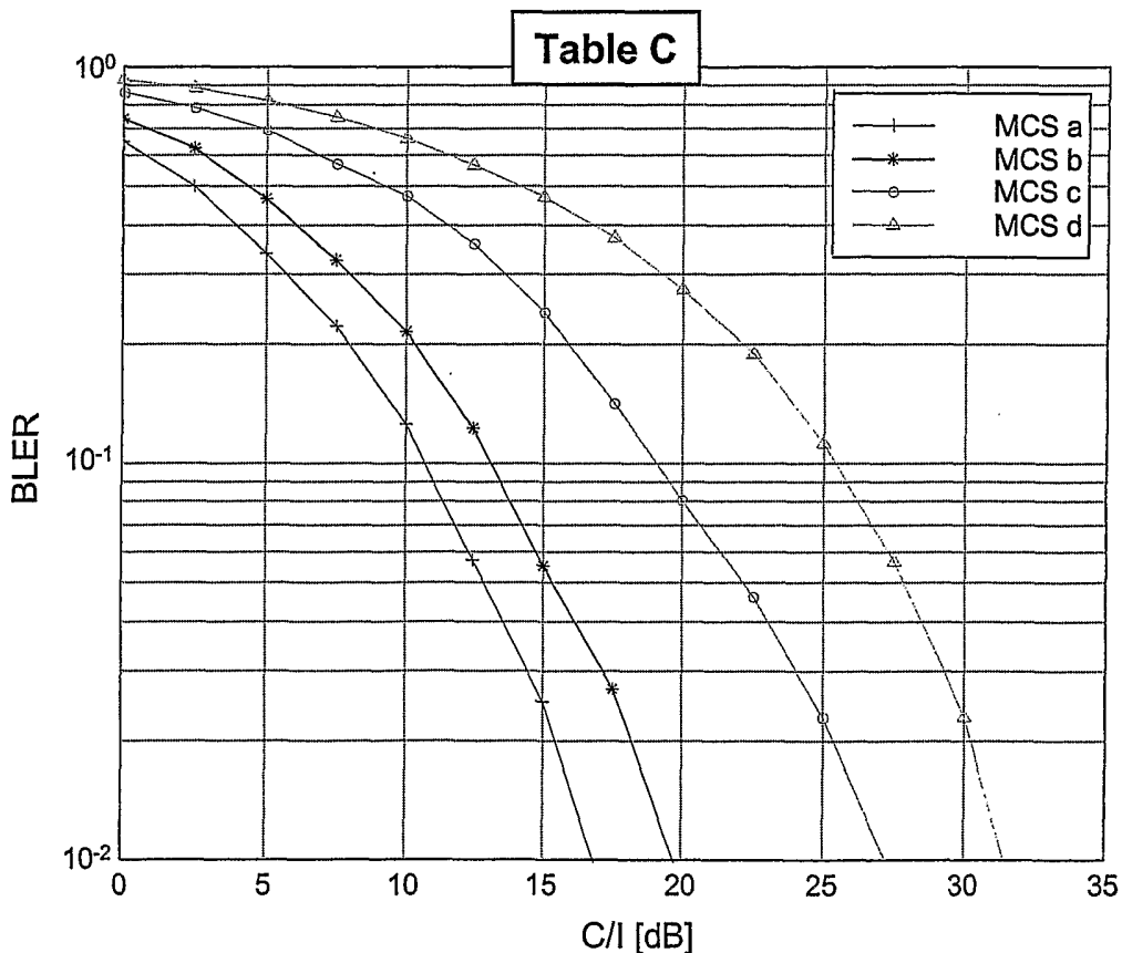
FIG. 12 BLER versus C/I for a selection of MCS (low diversity, with IR)
