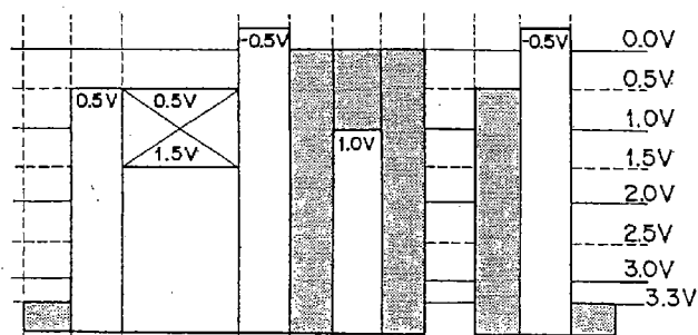
FIG. 5C t_6 < t NON-SELECTION STATE
