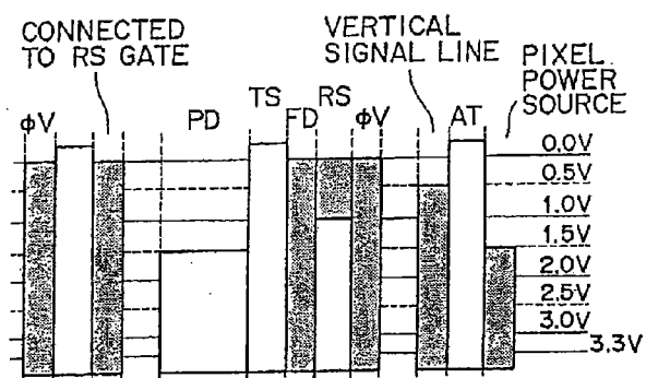
FIG. 13A t < t_1 NON-SELECTION STATE
