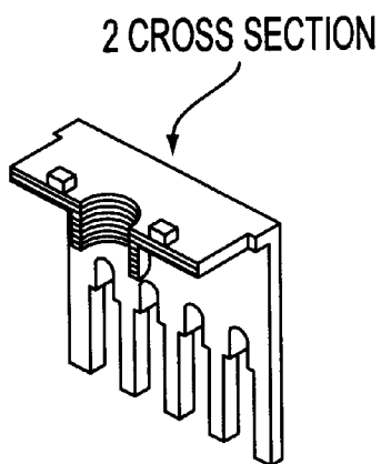
FIG. 6B (PRIOR ART)
