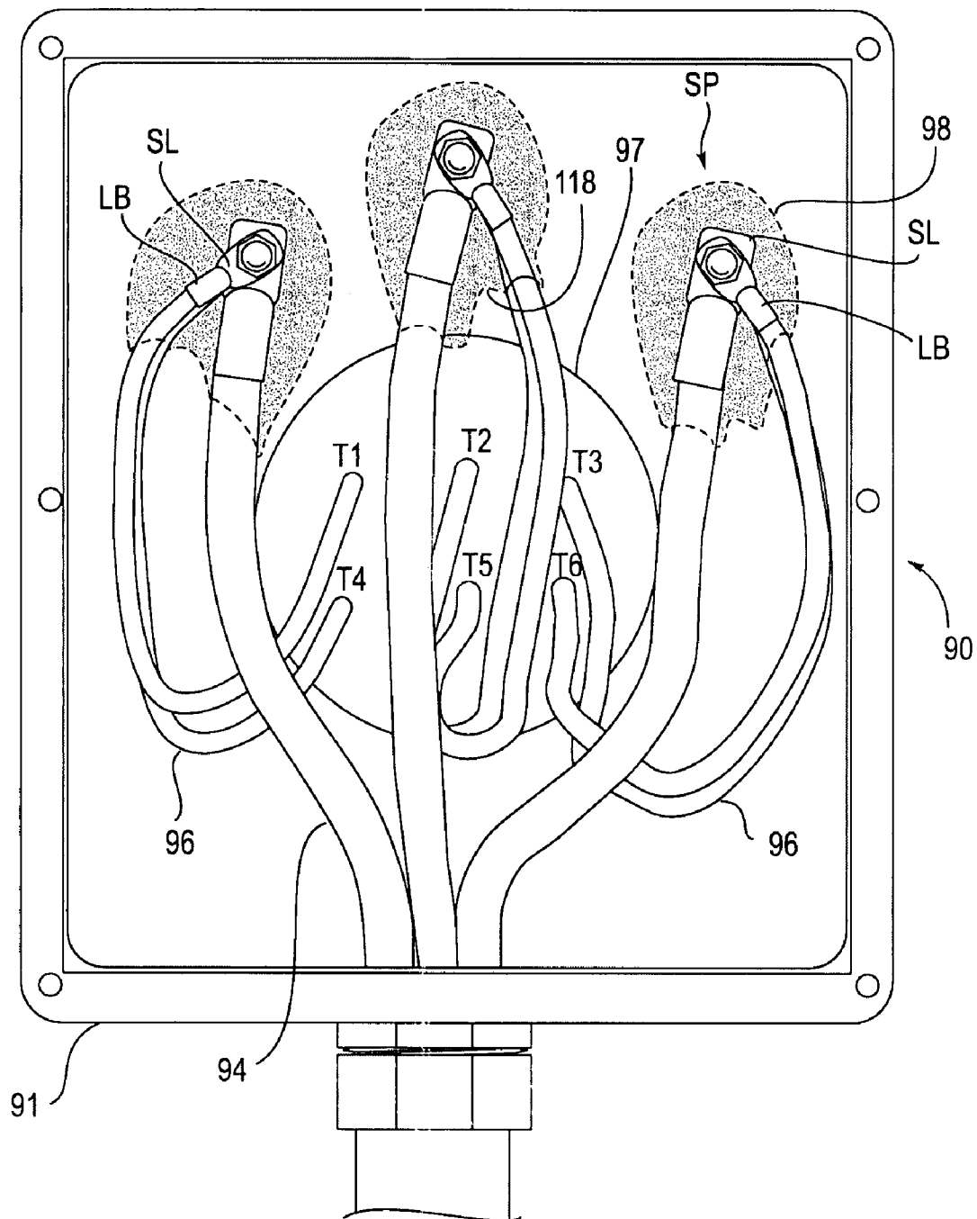
FIG. 10 (Prior Art)
