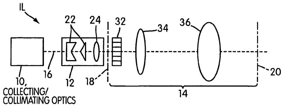
FIG. 7 (PRIOR ART)
