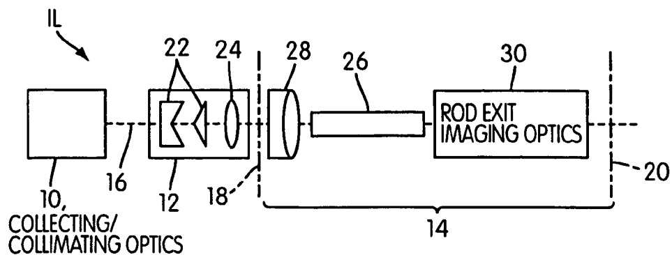
FIG. 6 (PRIOR ART)
