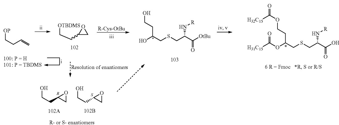
Scheme 5
