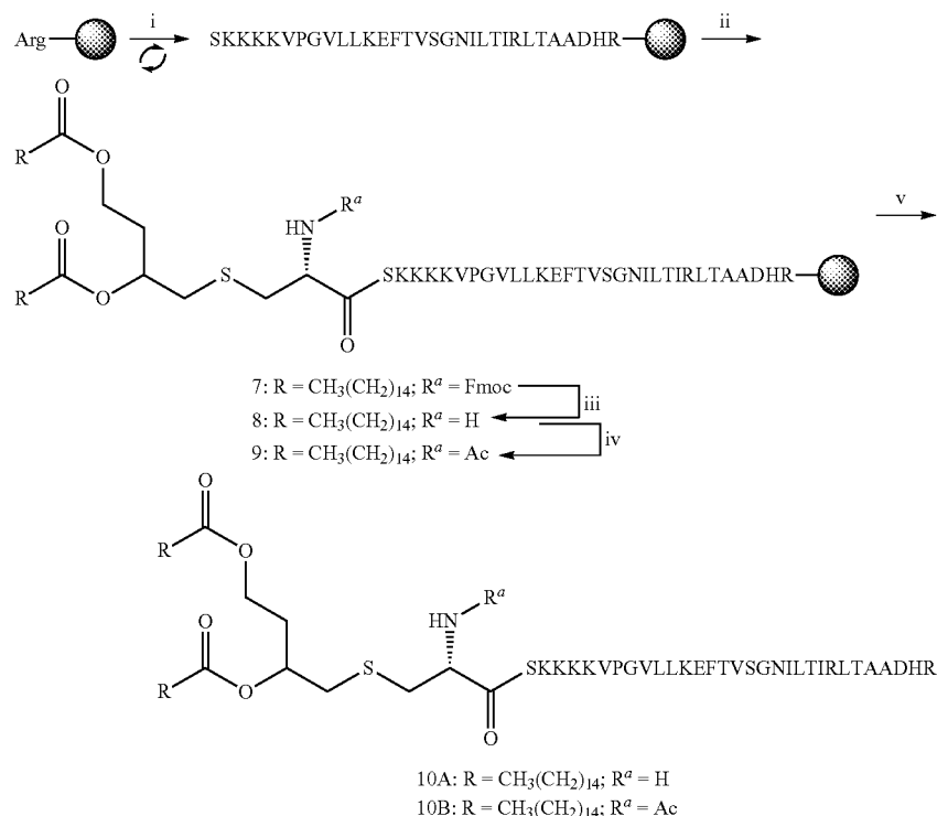
Scheme 6
