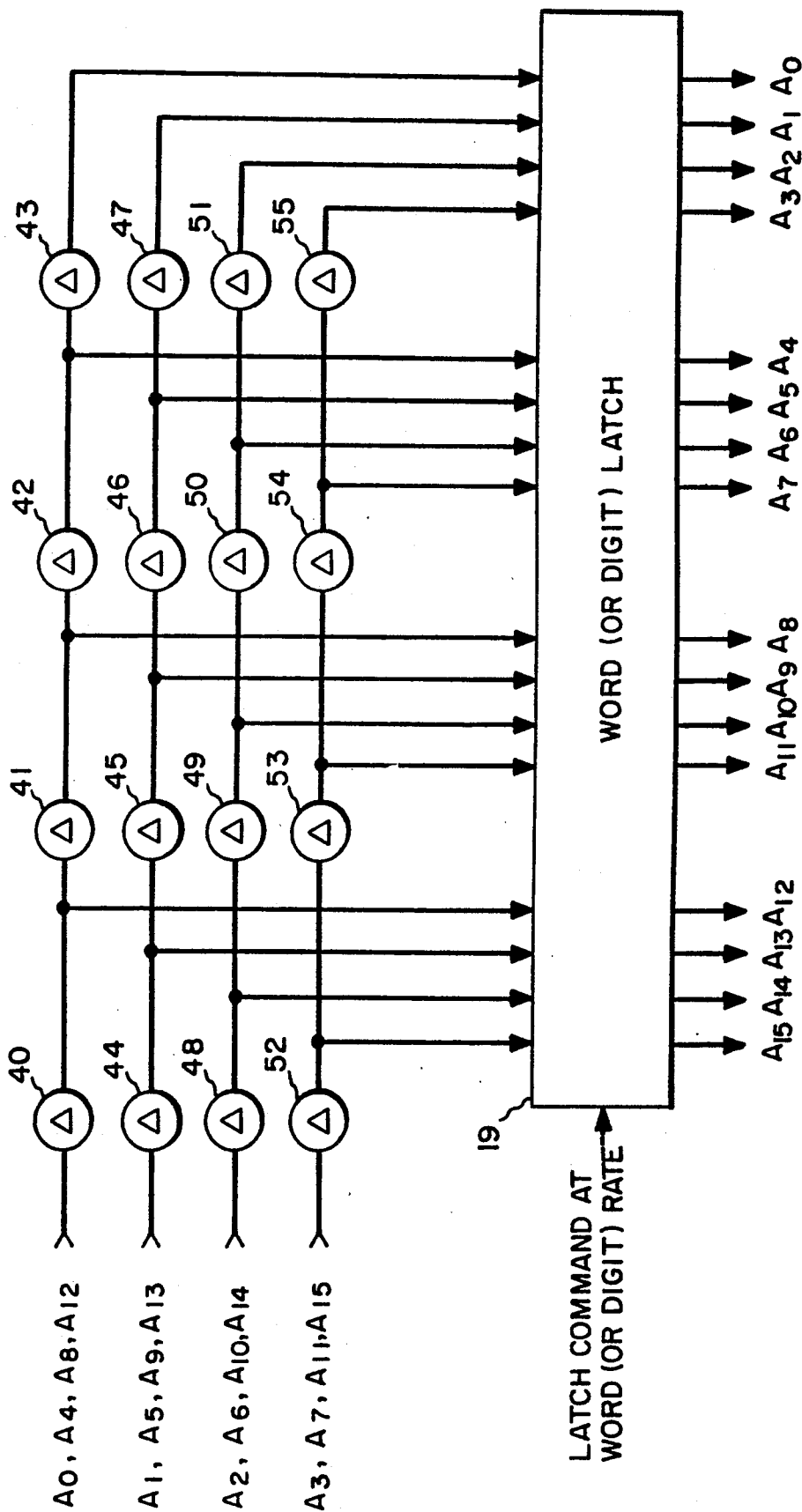
DIGIT-SERIAL-TO-PARALLEL CONVERTER (ADAPTABLE TO DIGIT-SERIAL-TO-DIGIT-SERIAL CONVERTER BY USING LATCH COMMAND AT DIGIT RATE)
