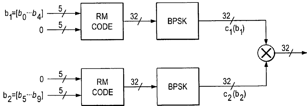
FIG. 5 (PRIOR ART)
