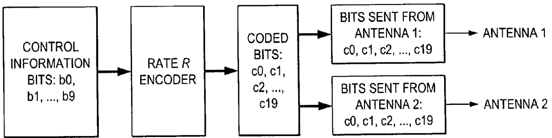
FIG. 7 (PRIOR ART)
