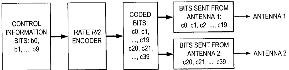
FIG. 8 (PRIOR ART)
