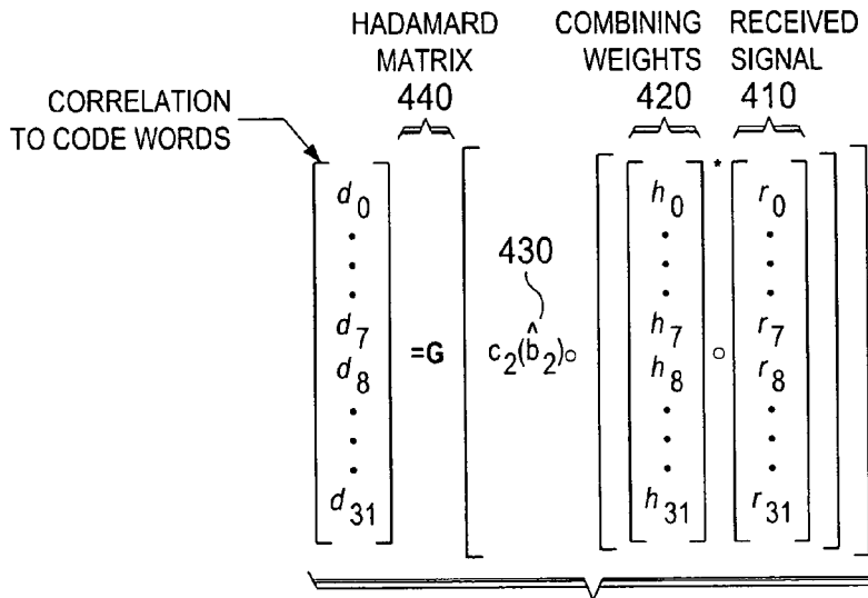
FIG. 4 (PRIOR ART)
