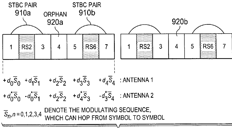
FIG. 9 (PRIOR ART)
