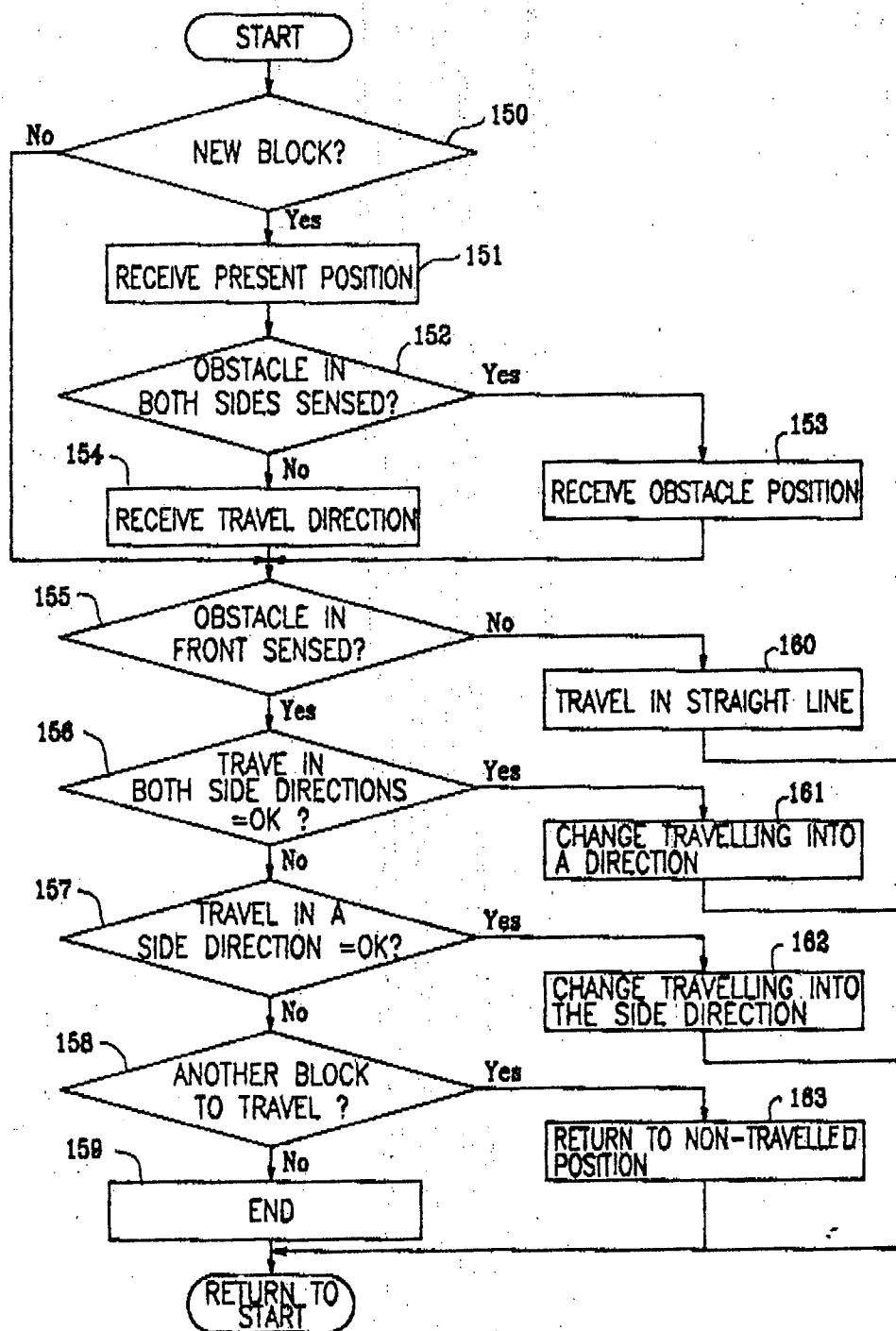
FIG. 13 PRIOR ART
