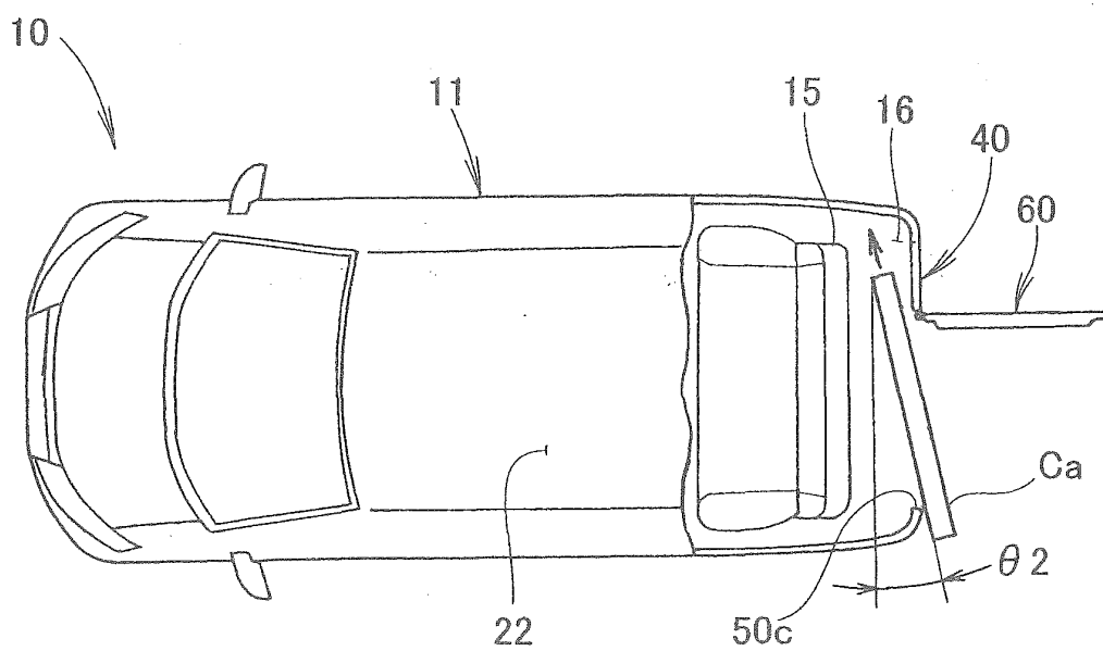
(b) EMBODIMENT
