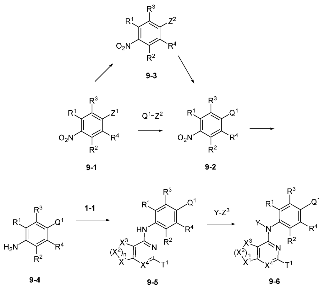
Scheme 9
