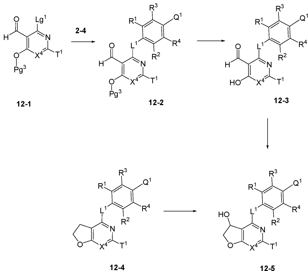
Scheme 12
