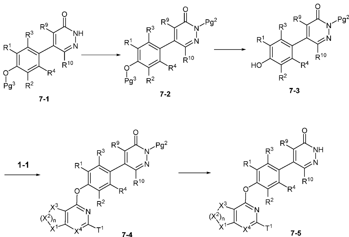
Scheme 7
