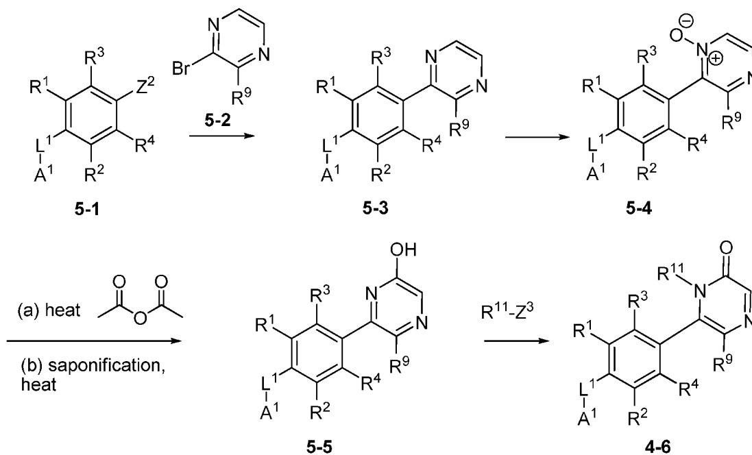
Scheme 5
