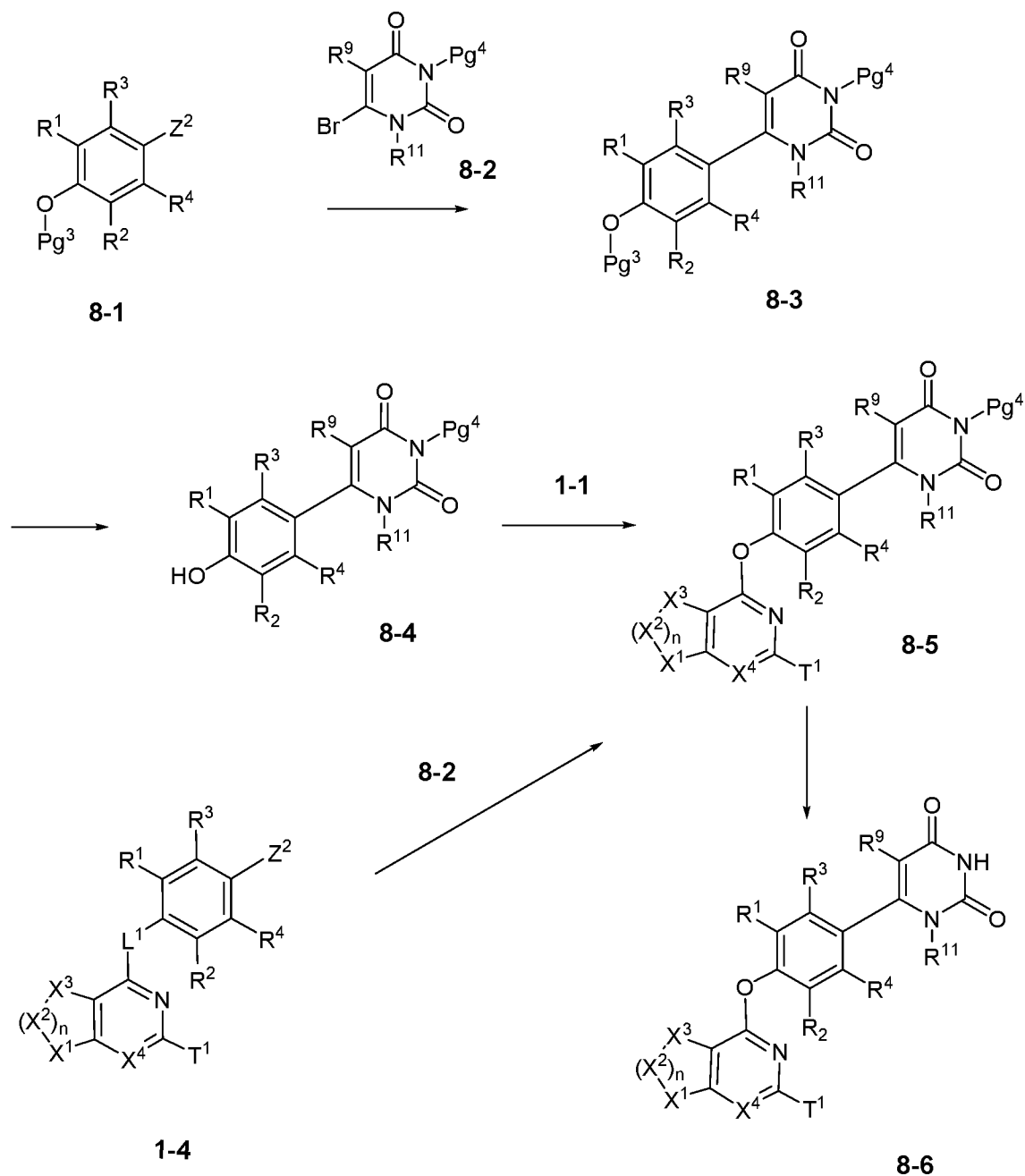
Scheme 8
