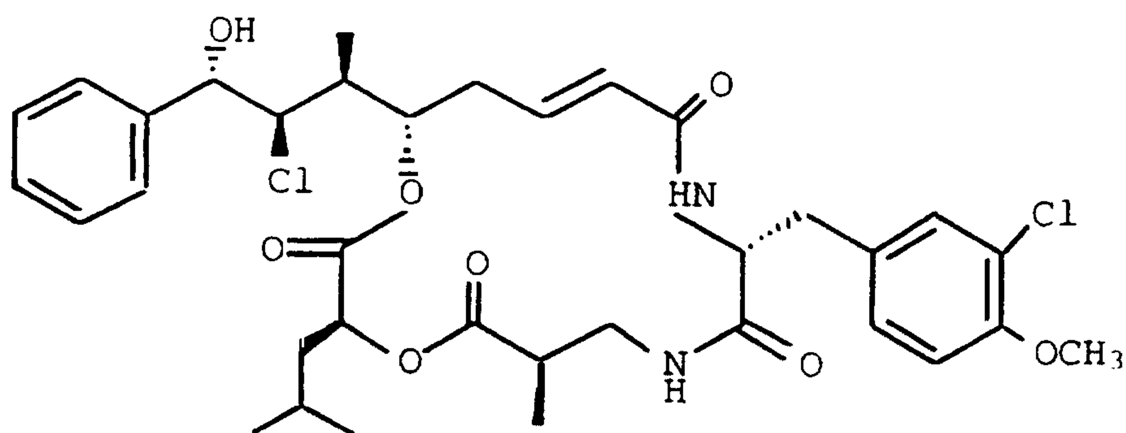
CRYPTOPHYCIN-140
