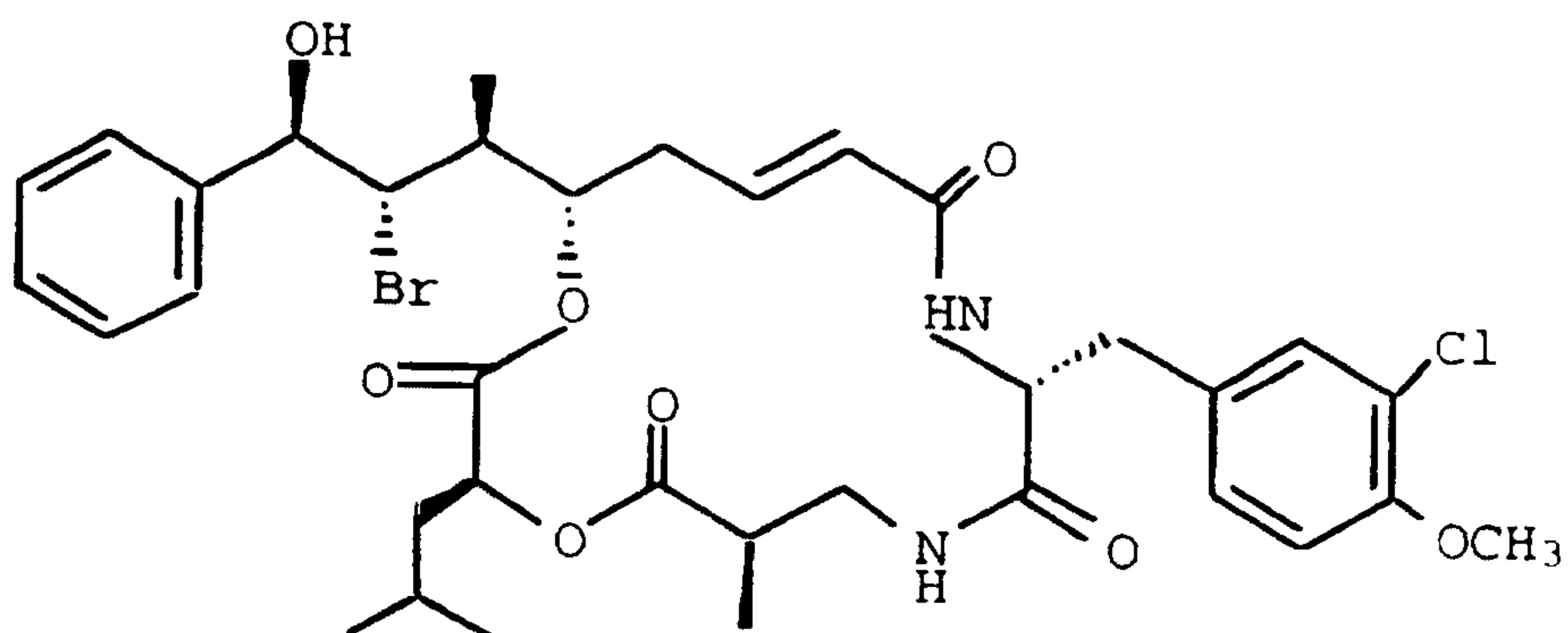
CRYPTOPHYCIN-145
