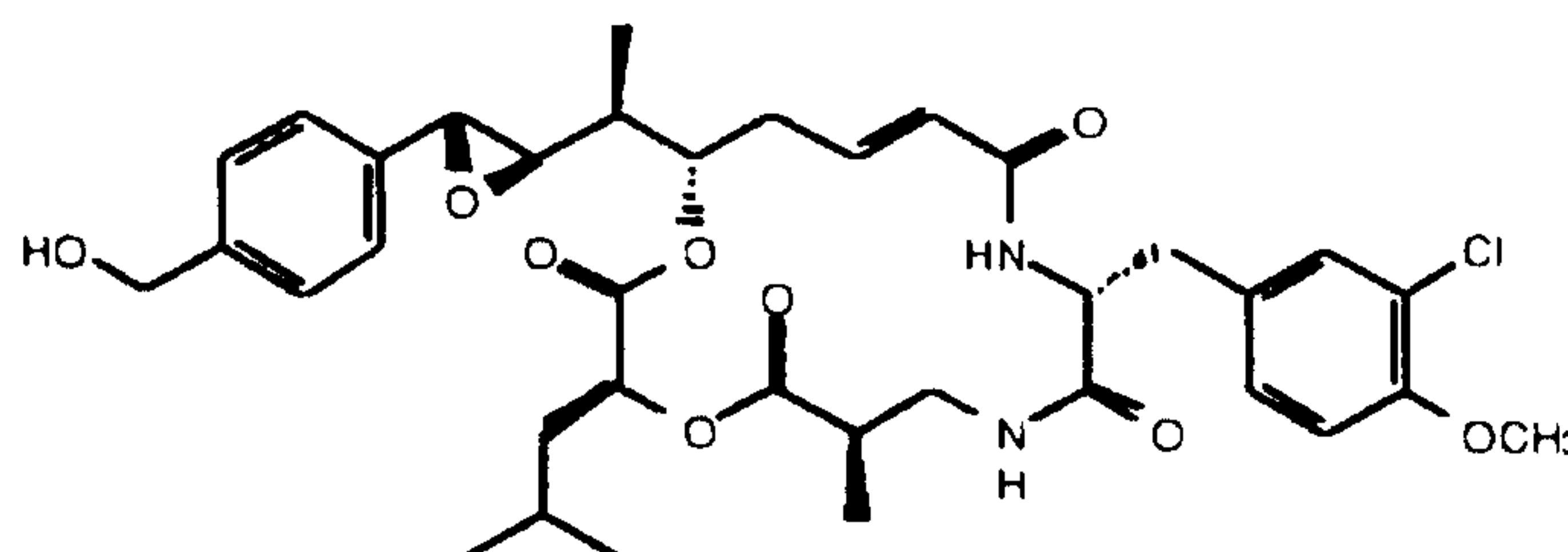
Cryptophycin-269
