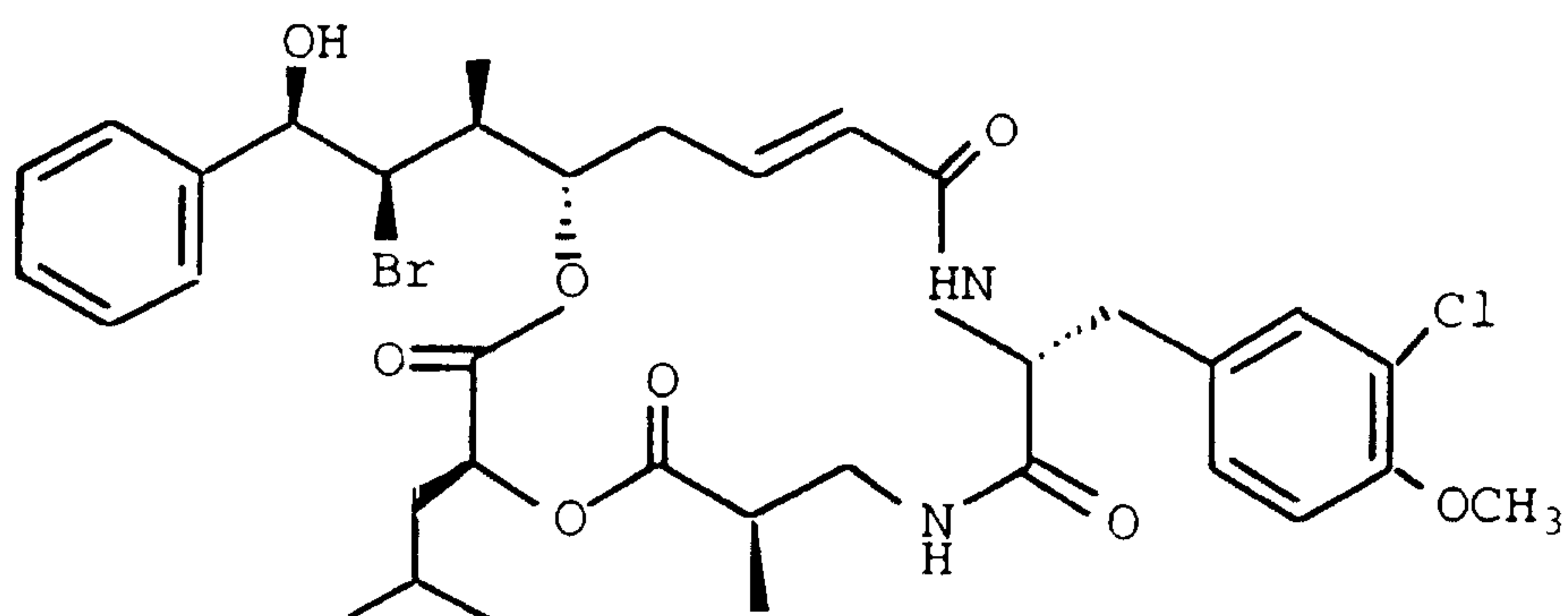
CRYPTOPHYCIN-138
