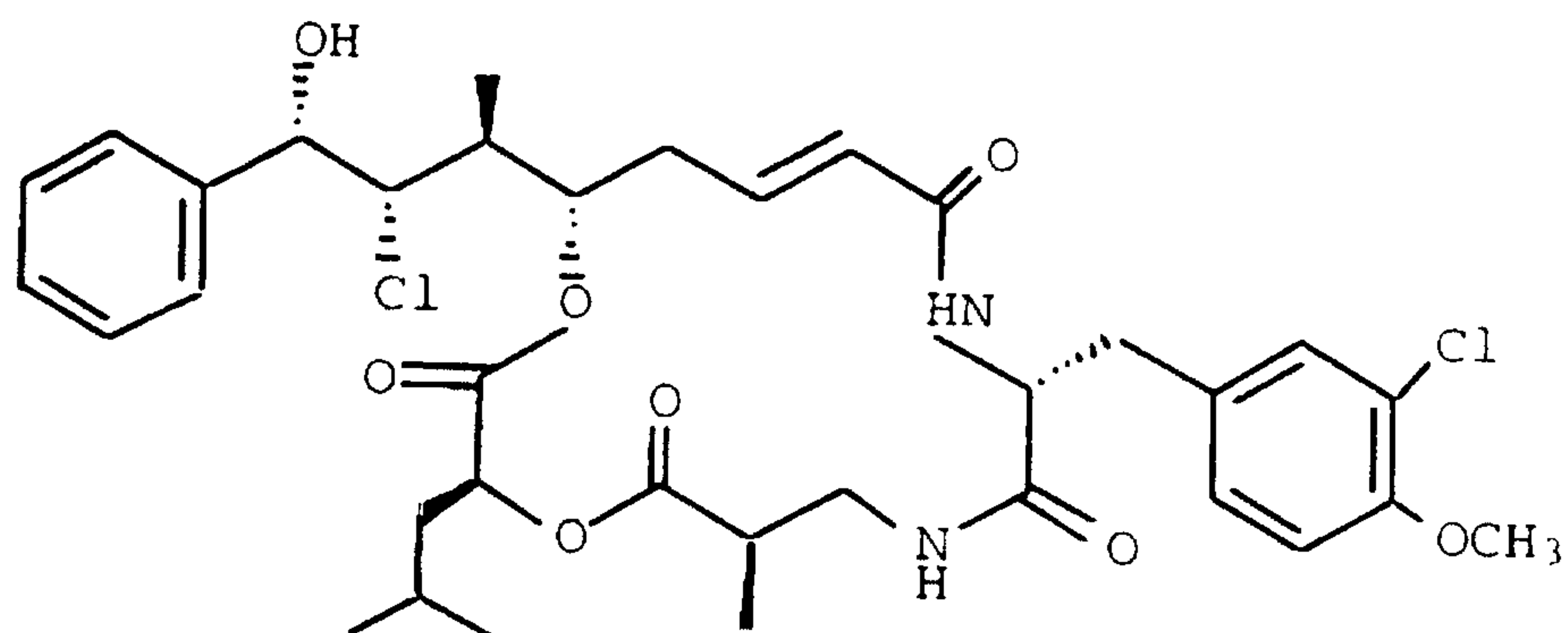
CRYPTOPHYCIN-143
