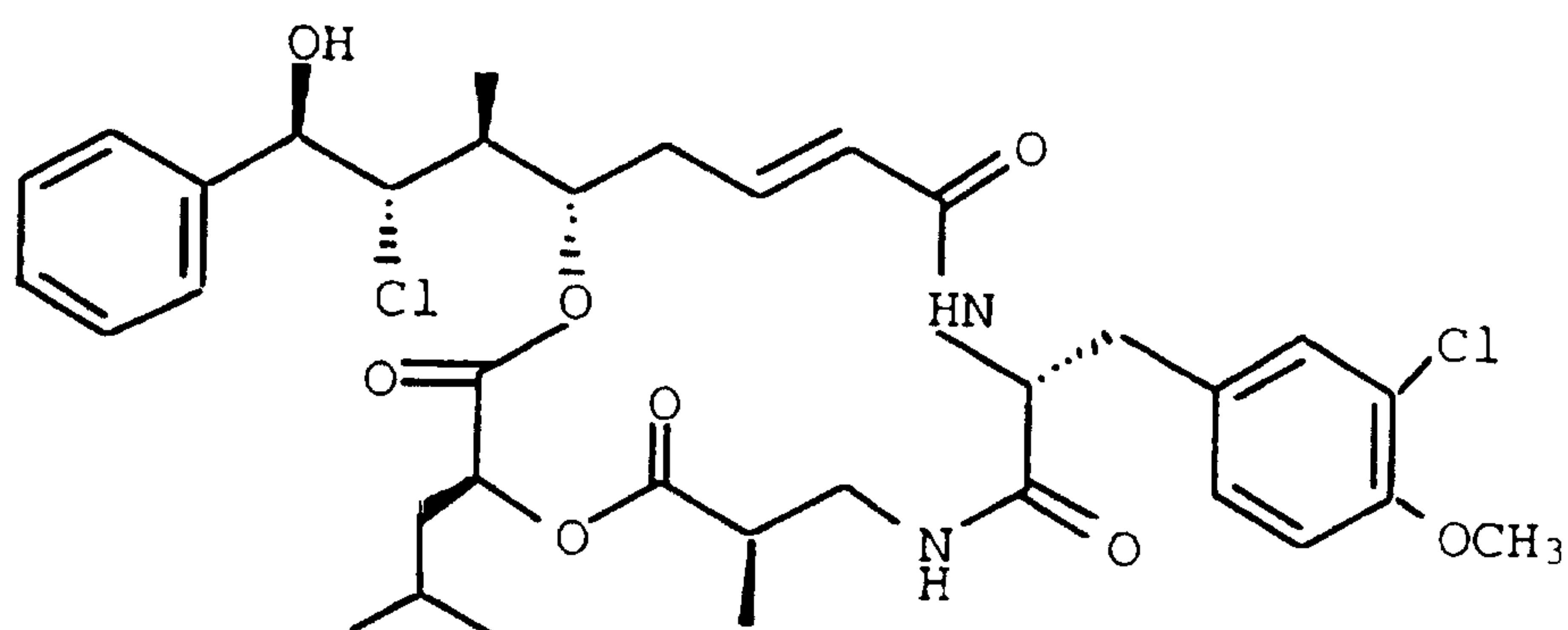
CRYPTOPHYCIN-142
