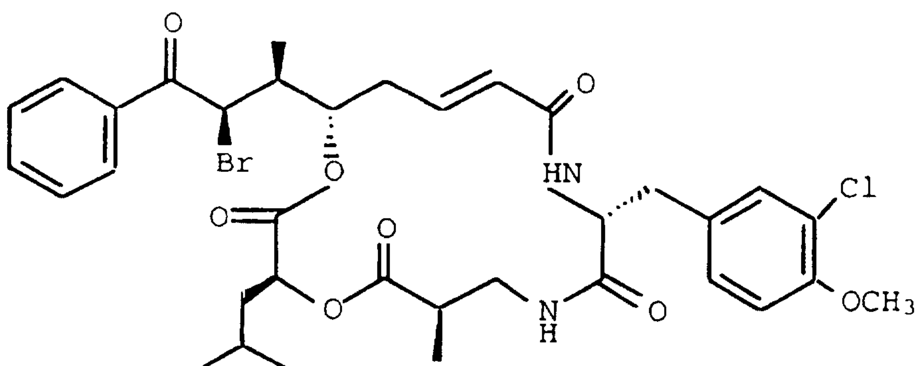
CRYPTOPHYCIN-139
