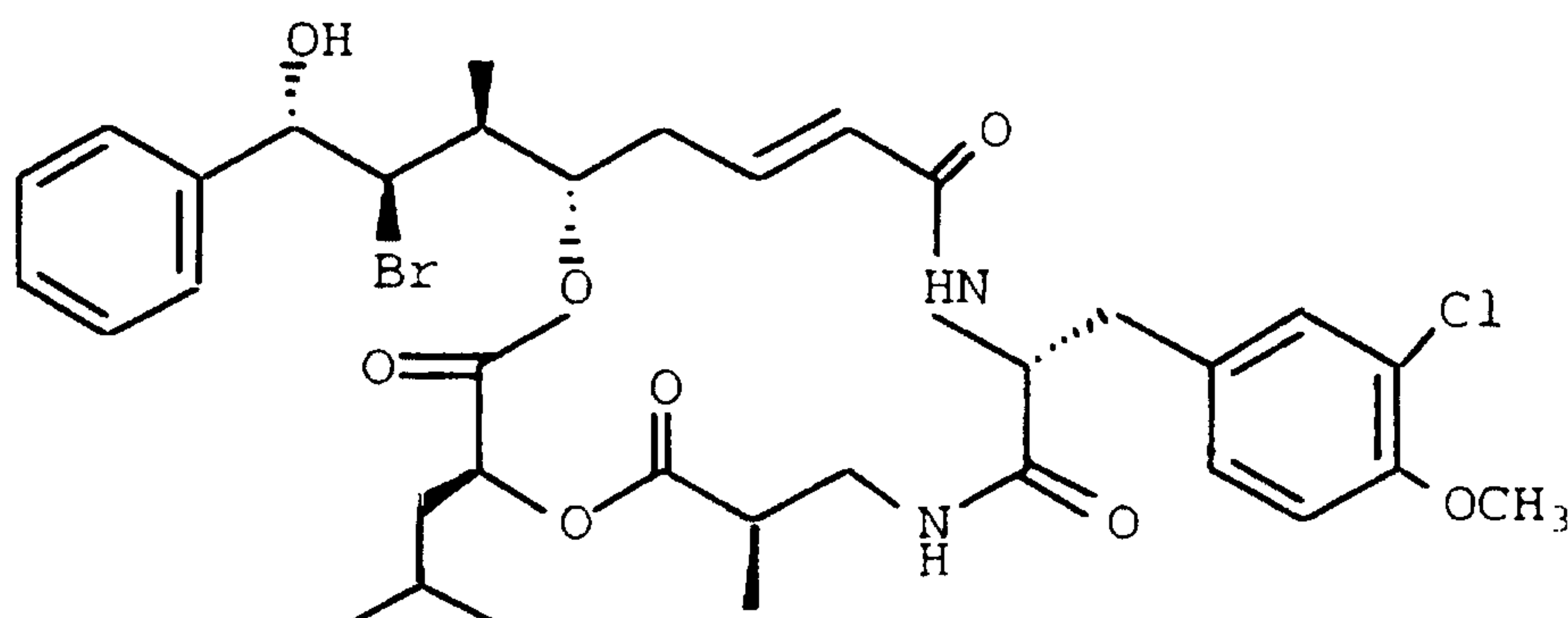
CRYPTOPHYCIN-129
