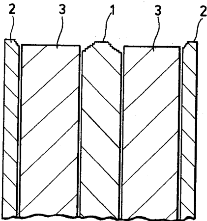
FIG.2. Prior Art Igniter After Failure
