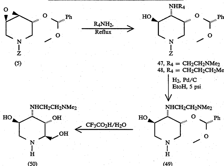
Scheme H: Synthesis of 3-amino 1,5-iminosugars.
