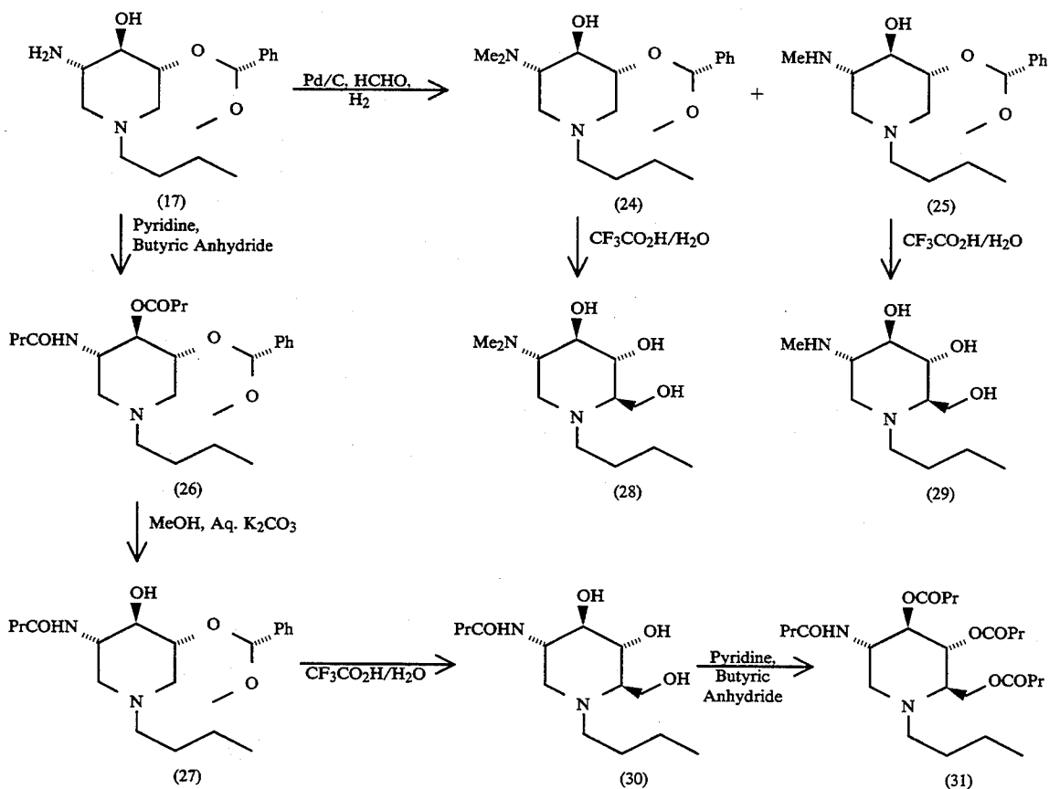
Scheme C: Synthesis of 2-alkylamino &amp; 2-acylamido 1,5-iminosugars.
