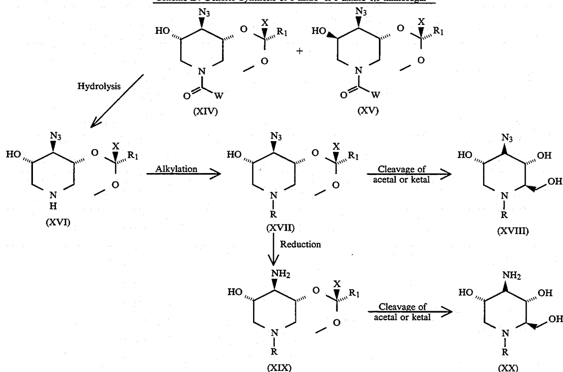
-continued Scheme D: Generic Synthesis of 3-azido- & 3-amino-1,5-iminosugar
