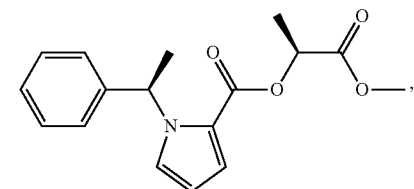
(R-methyl-MOC-carbometomidate)
