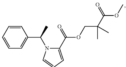
(α-dimethyl-MOC-carboetomidate)
