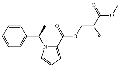
(α-S-methyl-MOC-carboetomidate)
