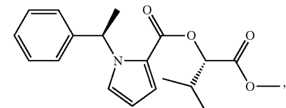
(S-isopropyl-MOC-carbometomidate)
