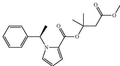
(β-dimethyl-MOC-carboetomidate)
