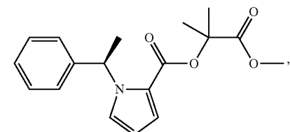
(dimethyl-MOC-carbometomidate)
