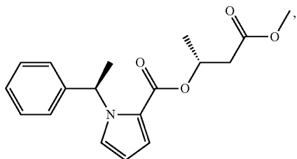
(β-S-methyl-MOC-carboetomidate)
