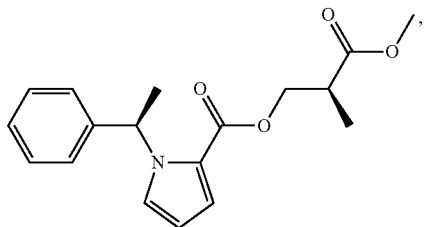
(α-R-methyl-MOC-carboetomidate)
