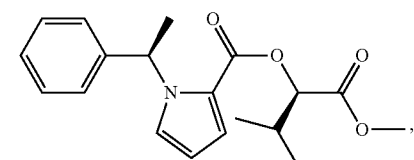
(R-isopropyl-MOC-carbometomidate)
