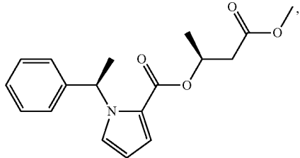
(β-R-methyl-MOC-carboetomidate)
