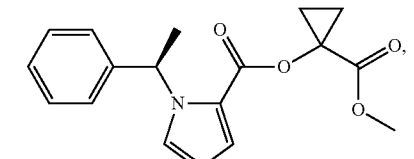
(cyclopropyl-MOC-carbometomidate)
