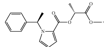
(S-methyl-MOC-carbometomidate)
