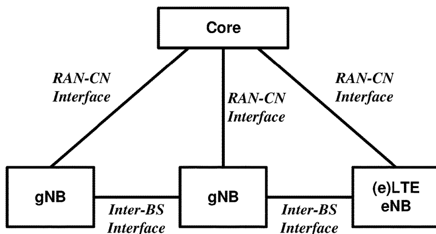
Non-centralized deployment
