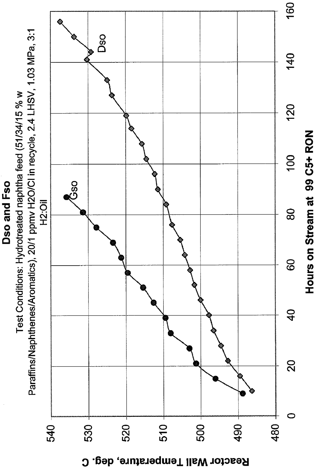
Figure 4. Activity Decline Data for Steamed and Oxychlorinated Catalysts
