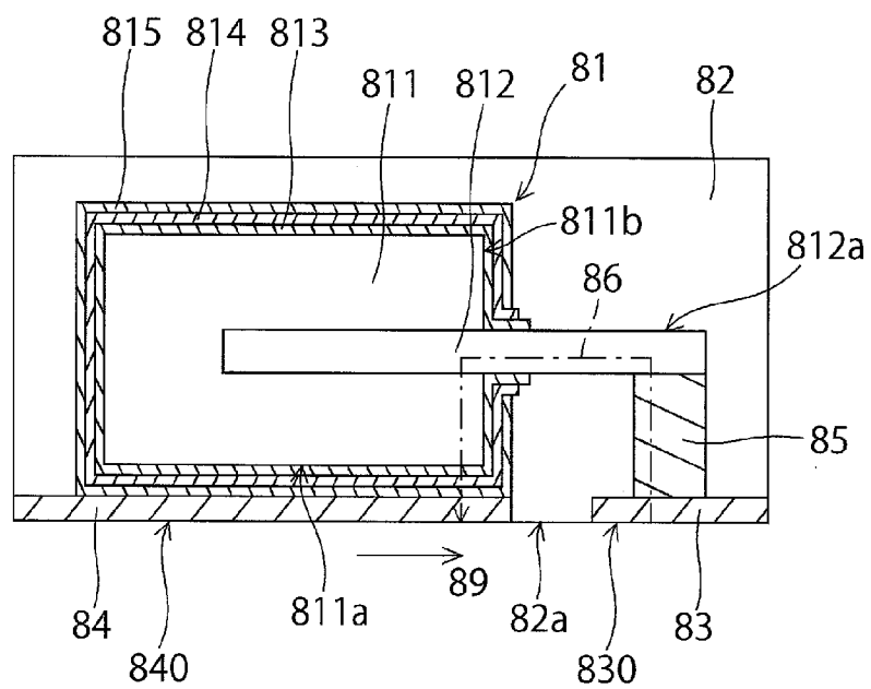
FIG.17 PRIOR ART
