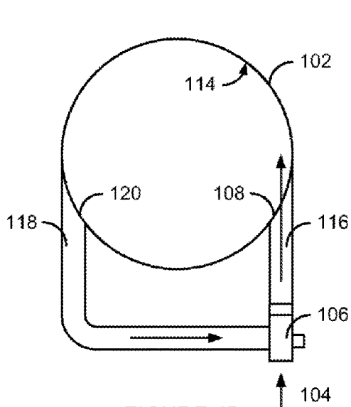
FIGURE 1B CROSS SECTION E-E
