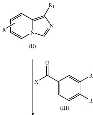
Scheme 1
