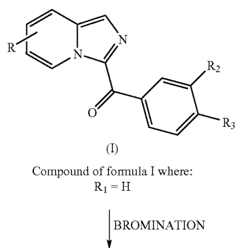
Scheme 3
