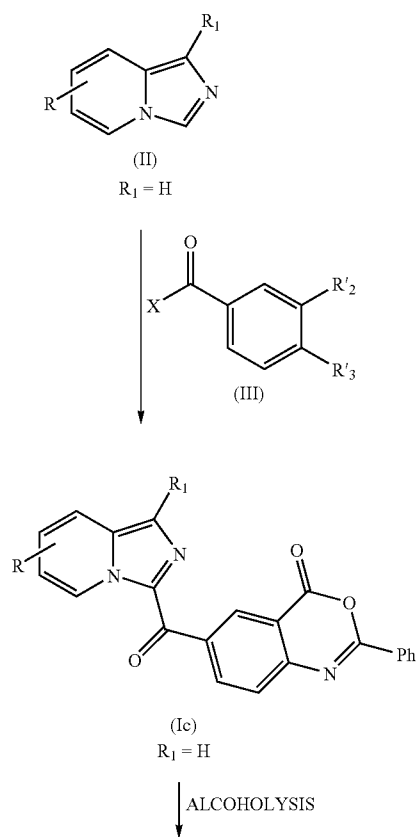
Scheme 2
