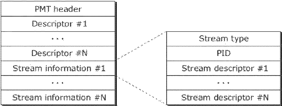
Data structure of PMT
