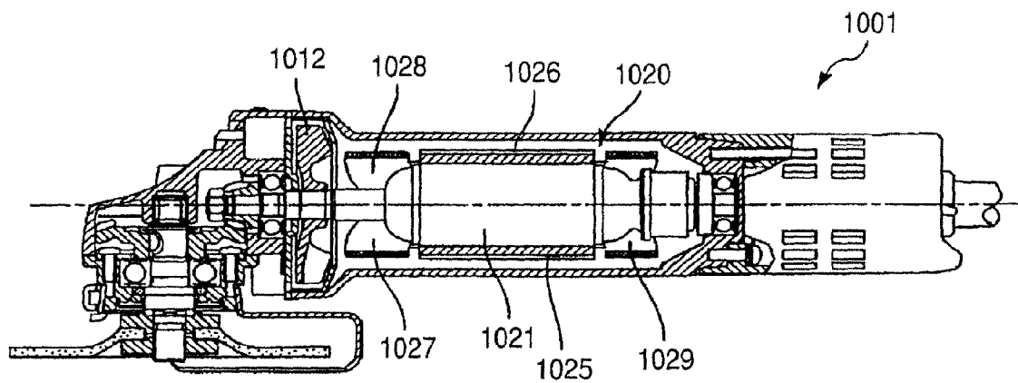
FIG. 13 PRIOR ART
