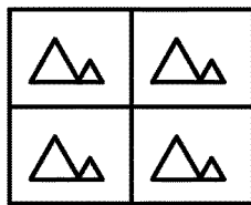
Grid View
