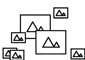
Scatter View
