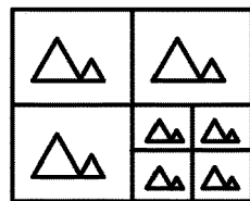
Multiscale Grid
