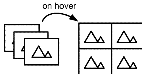
Stack-and-Hover View
