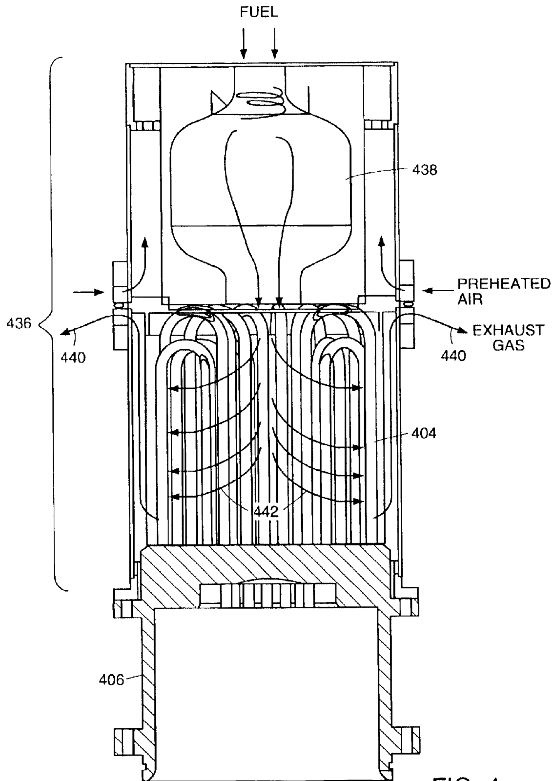
FIG. 4 PRIOR ART
