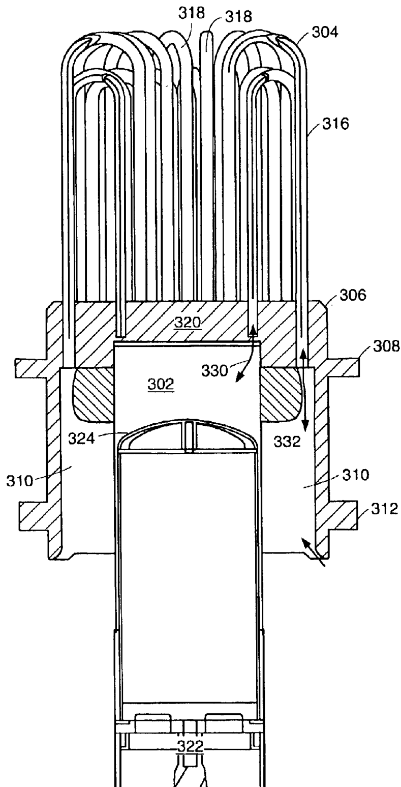
FIG. 3 PRIOR ART
