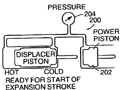
FIG. 2c PRIOR ART
