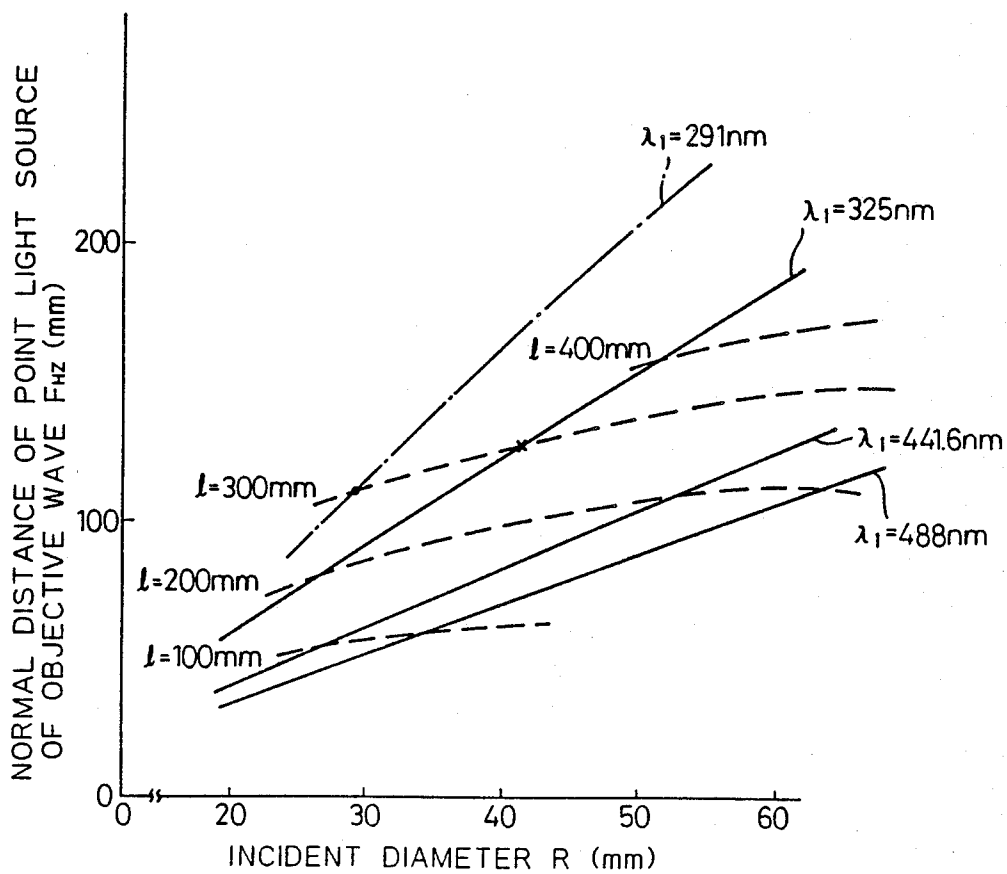
Fig. 15 (PRIOR ART)
